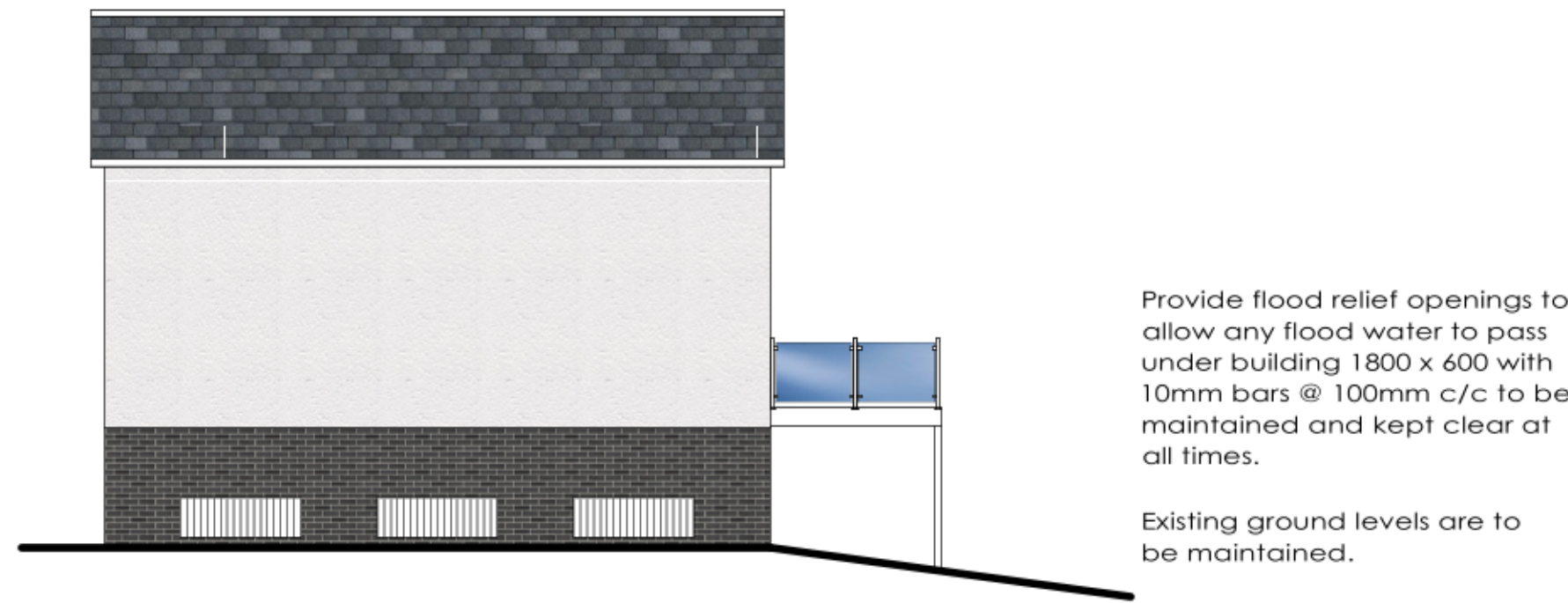
West Elevation
