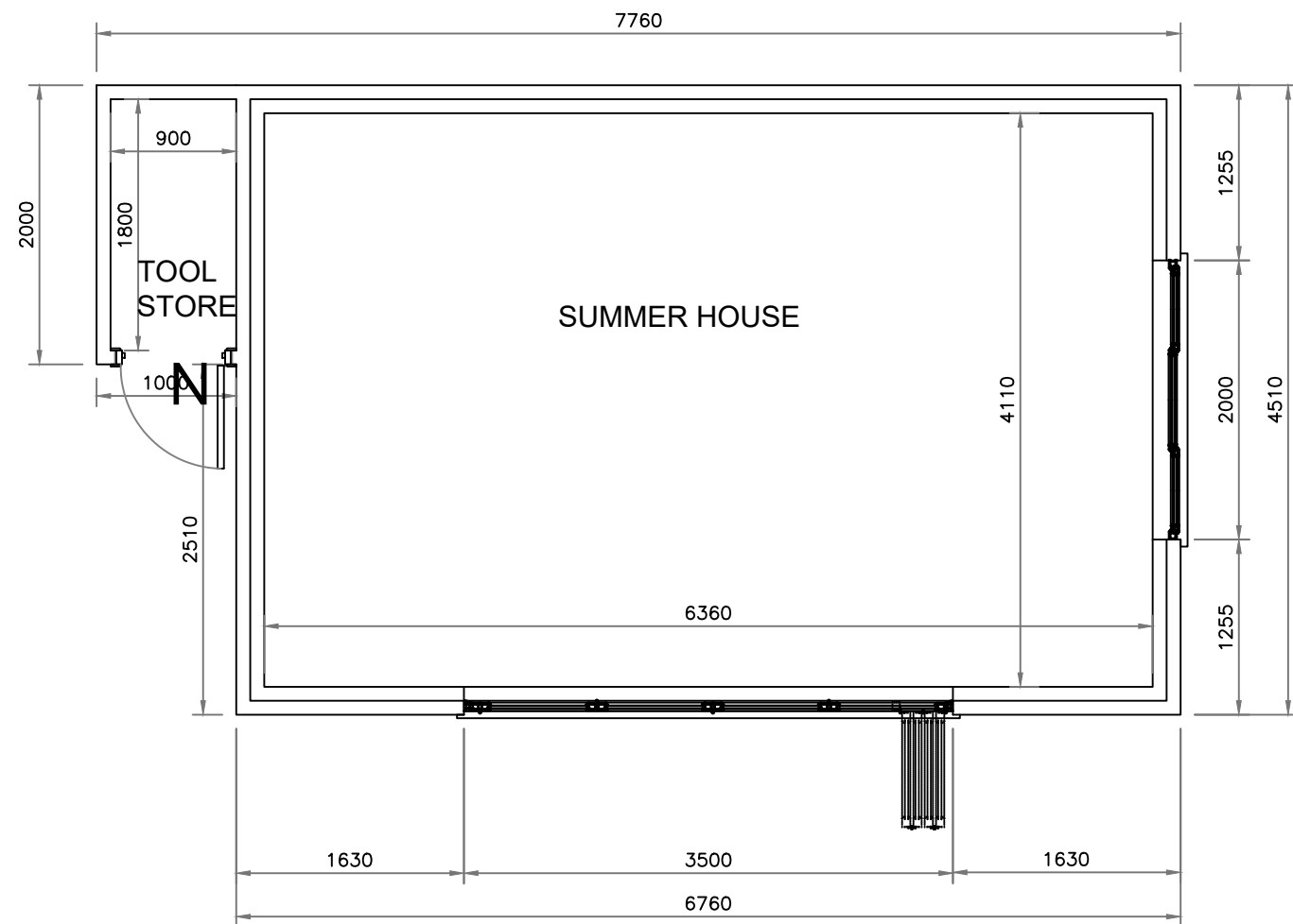
FLOOR PLAN 1:50
