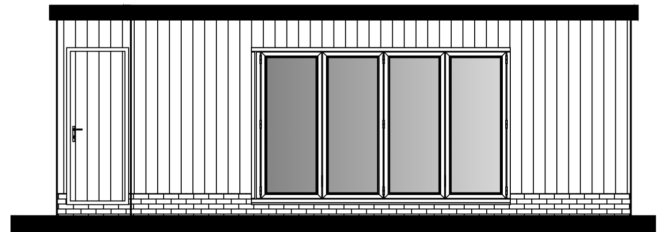
FRONT ELEVATION 1:50
