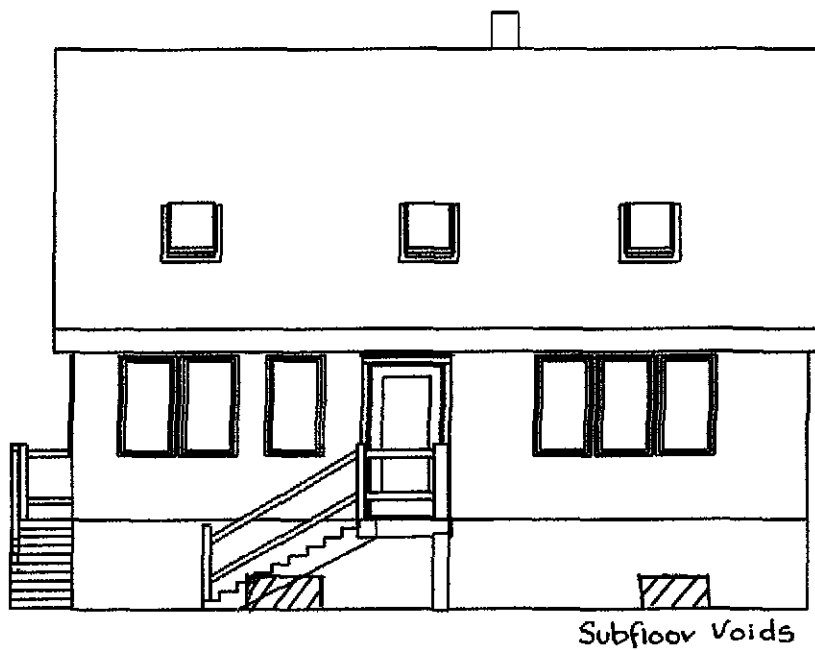
Proposed Rear Elevation 30 The Reservoir, Surfleet PE11 4DJ
