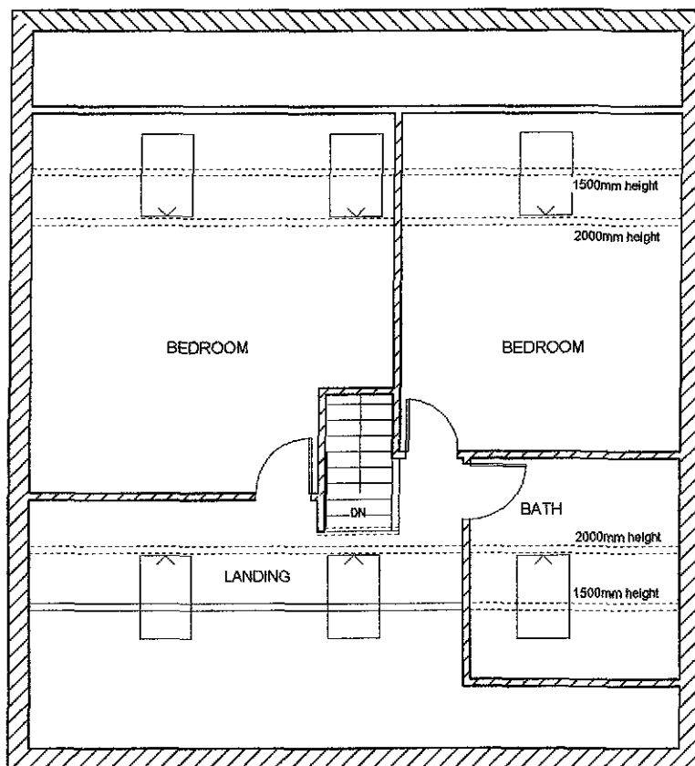
First Floor, 30 the Reservoir, PE11 4DJ
