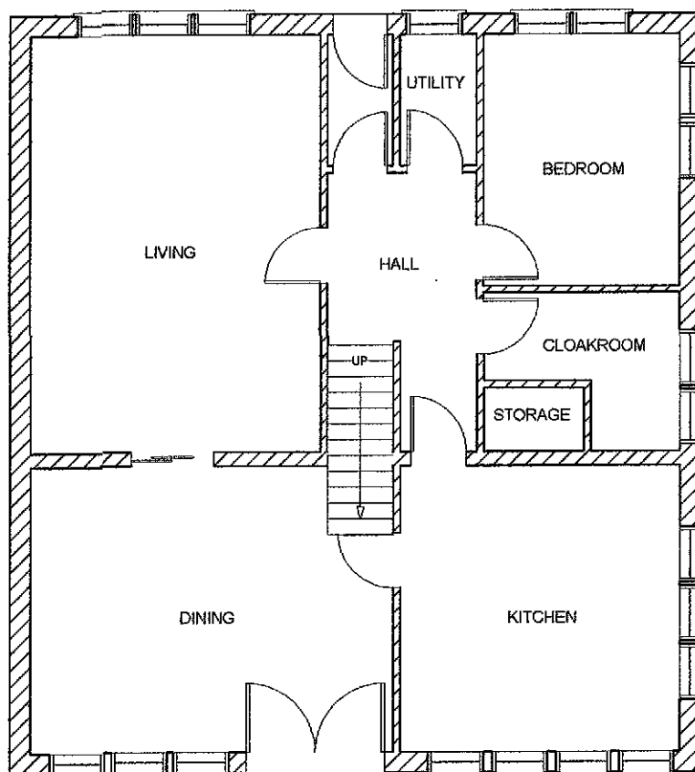
Ground Floor, 30 The Reservoir, PE11 4DJ
