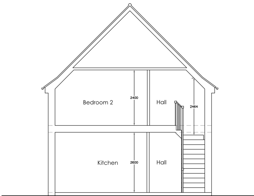
Section
