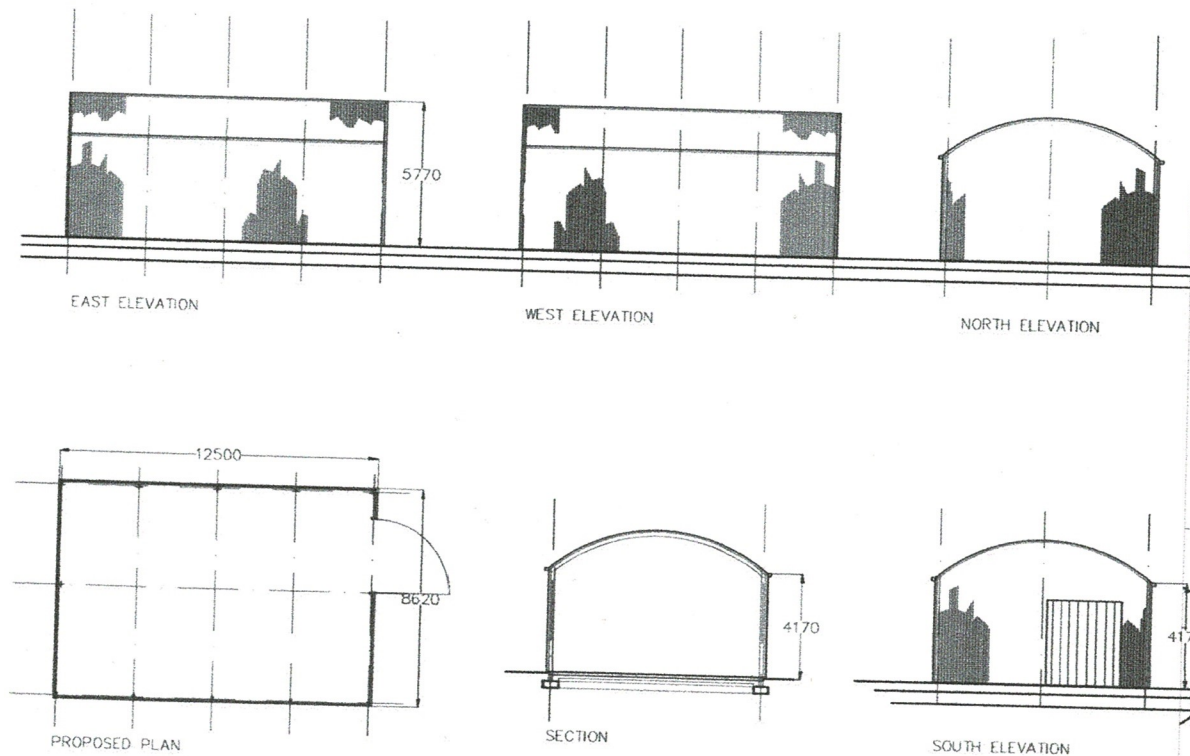
BUILDING PLANS SCALE 1/100
