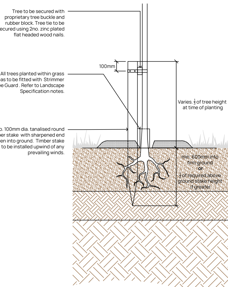
Detail 6 - Standard to Select Standard Support Detail
