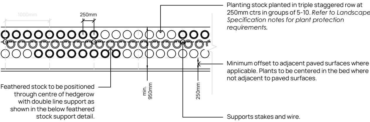
Detail 4 - Typical Native Hedgerow Triple Staggered Layout (N.T.S.)
