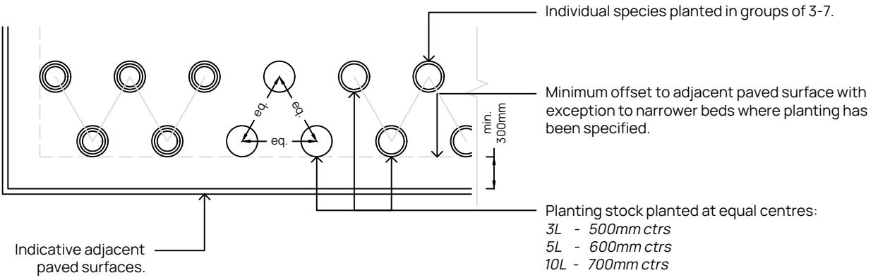
Detail 1 - Typical Shrub Planting Layout (N.T.S.)
