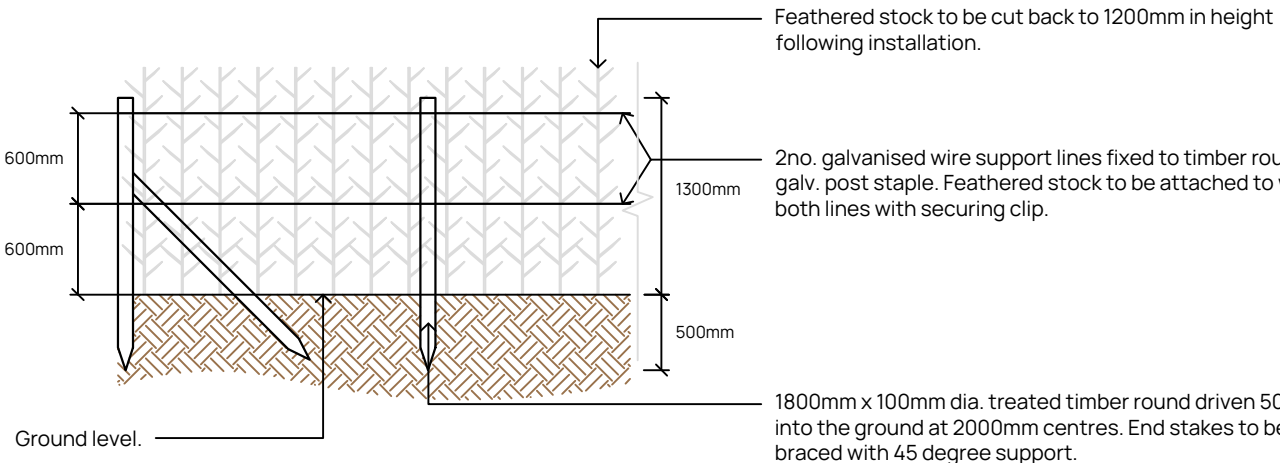
Detail 5 - Typical Feathered Stock Support Detail (N.T.S.)
