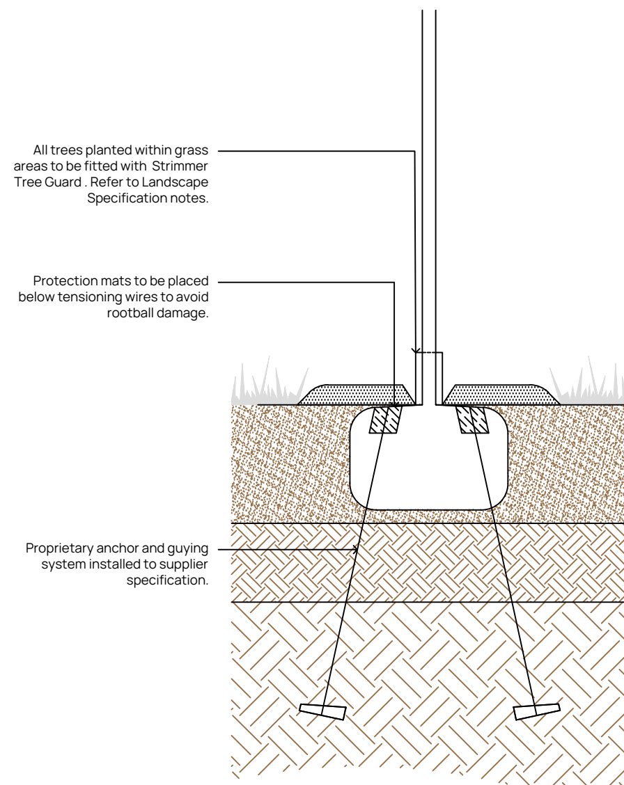
Detail 8 - Typical Semi Mature 25cm+ Girth Support Detail
