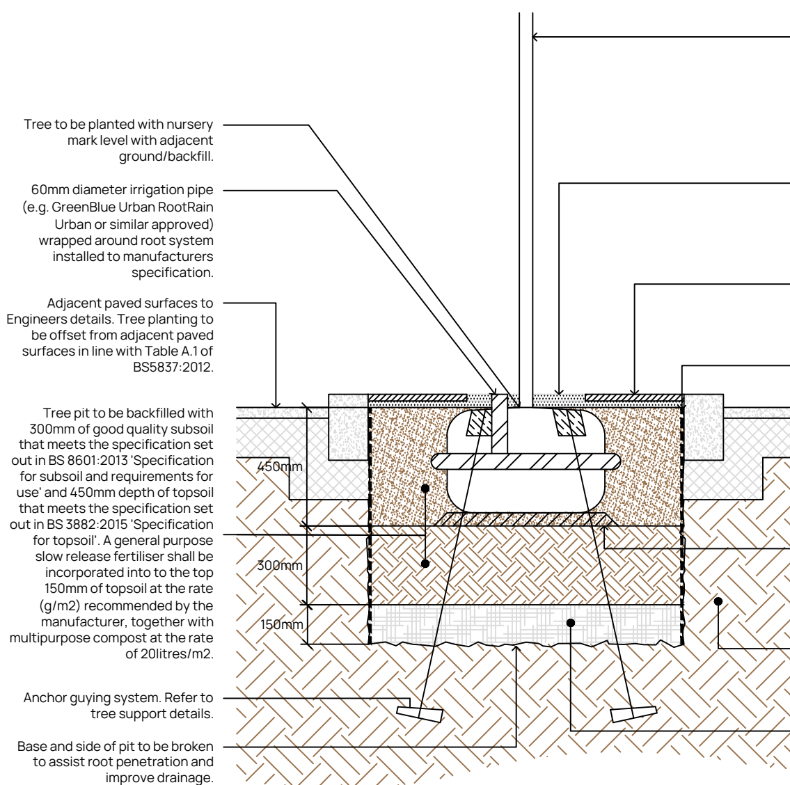
Detail 10 - Typical Tree Pit within Hard Landscape (N.T.S.)
