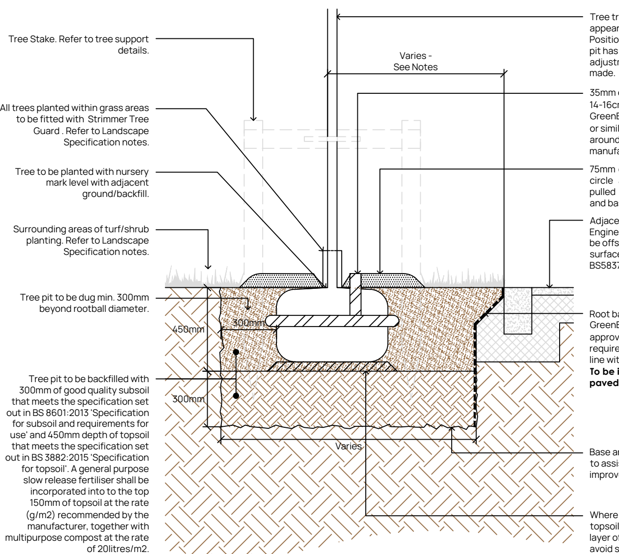
Detail 9 - Typical Tree Pit within Soft Landscape (N.T.S.)
