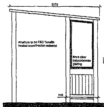
Side Elevations
