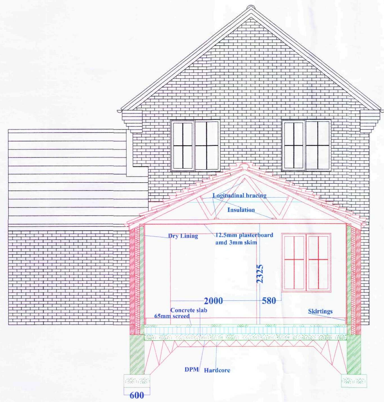
SECTION
