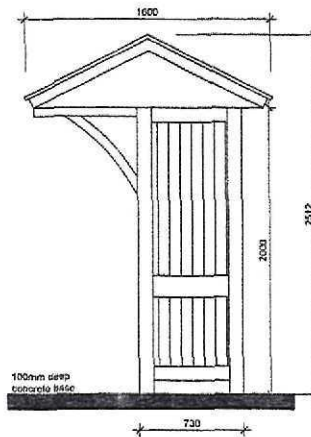
Side Elevations
