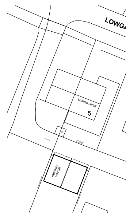
Block Plan
