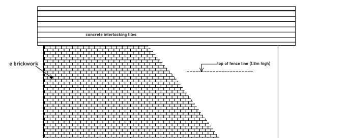
Left Side Elevations
