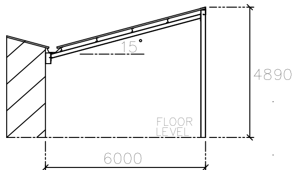
SECTION THROUGH
