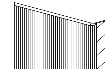
GABLE ELEVATION TO LINE 3
