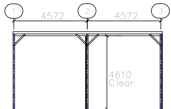
SIDE ELEVATION TO LINE A
