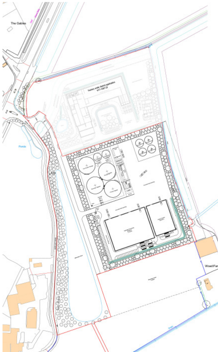
Figure 5 - Indicative Site Plan
