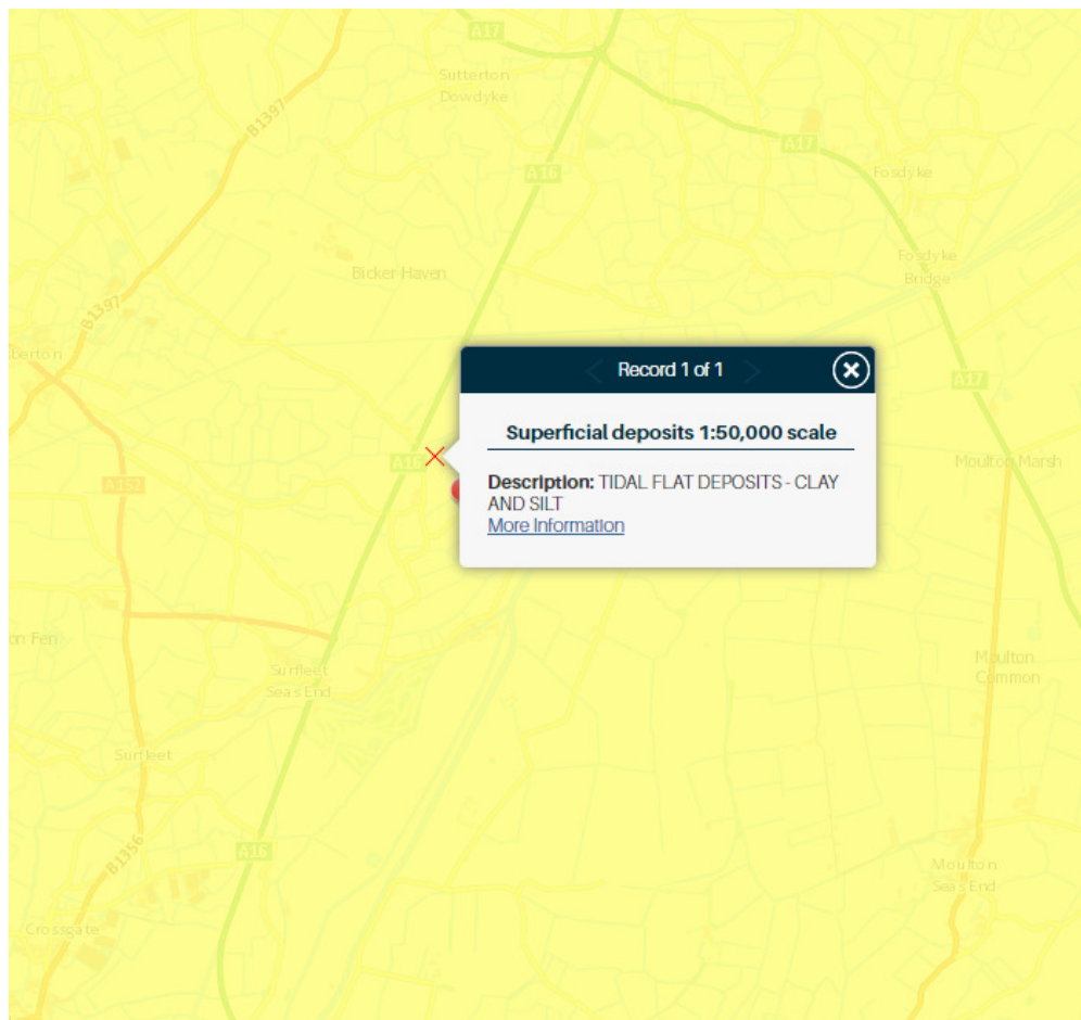
Figure 3 - BGS Superficial Deposits
