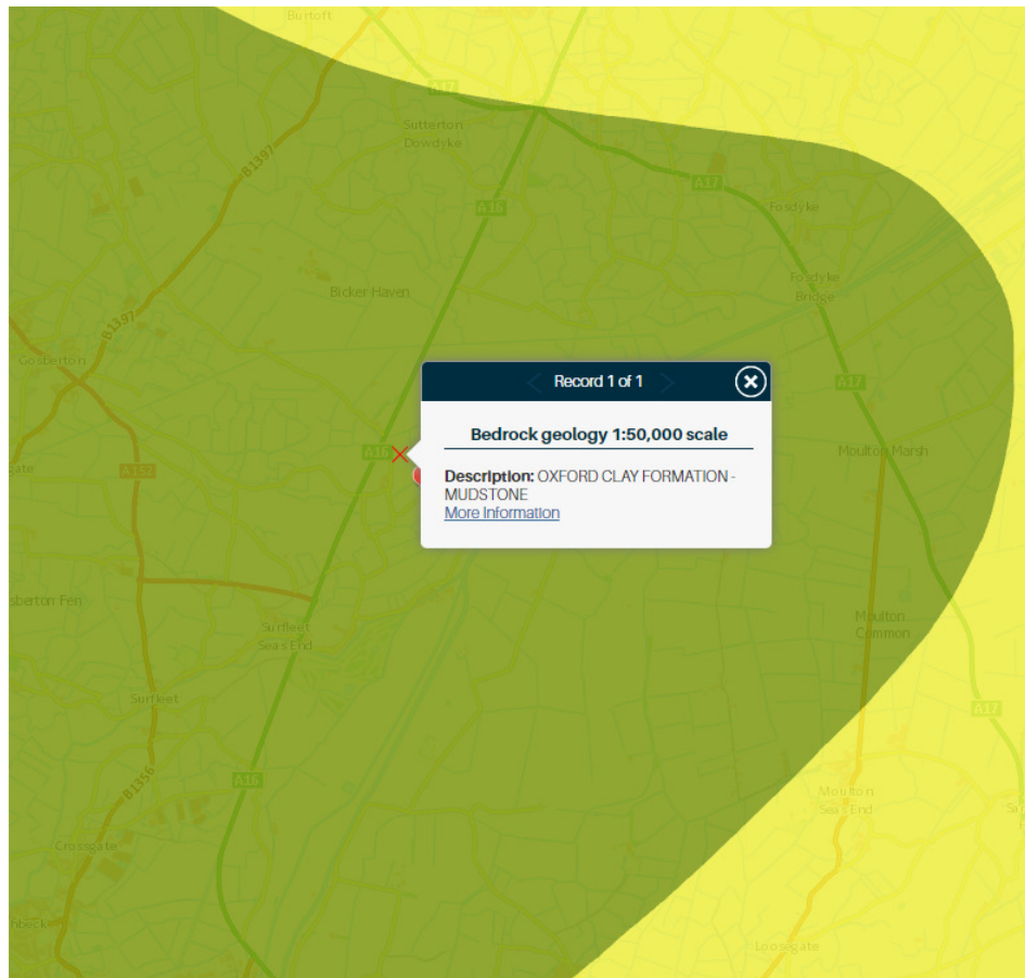
Figure 2 - BGS Bedrock Geology
