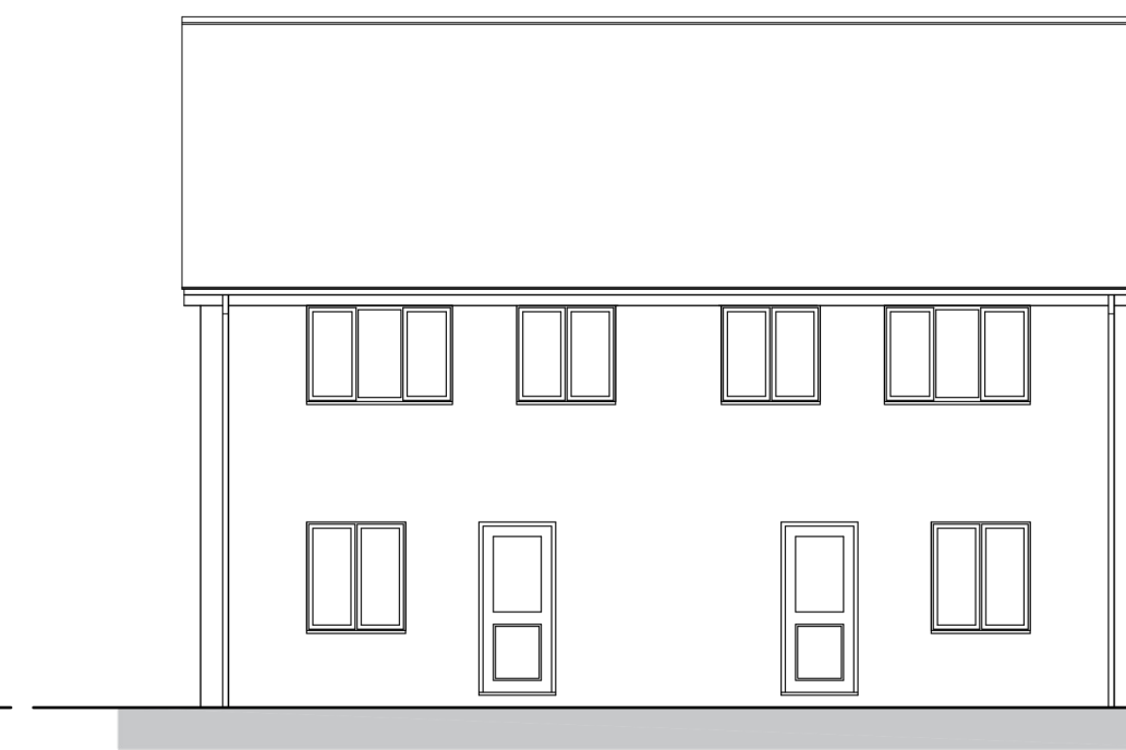
Rear Elevation
