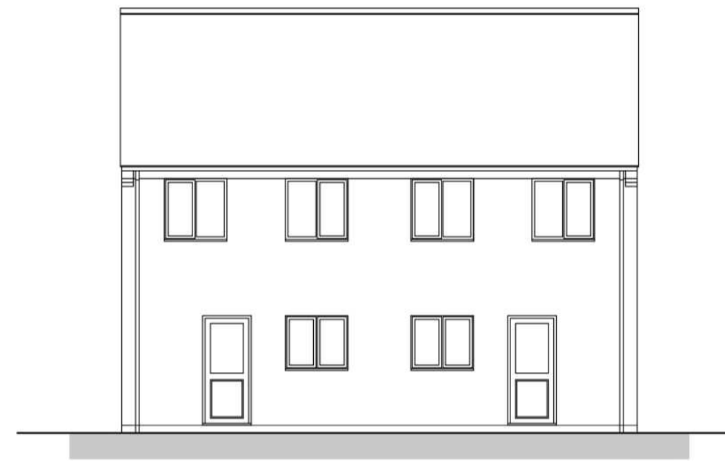
Rear Elevation
