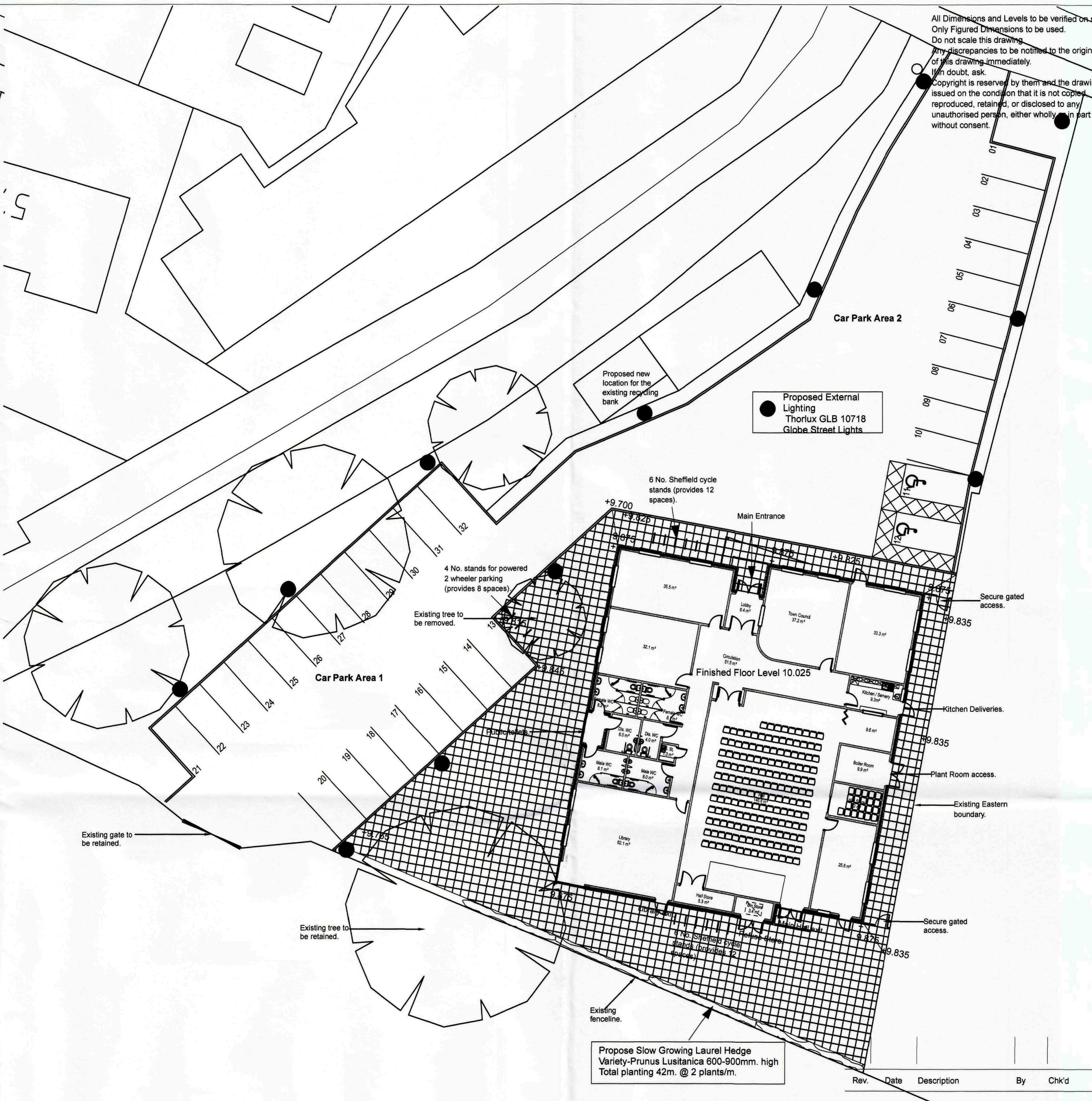
Proposed Site Levels 1:200
