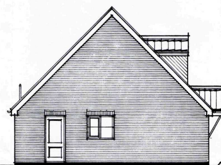
SIDE ELEVATION
