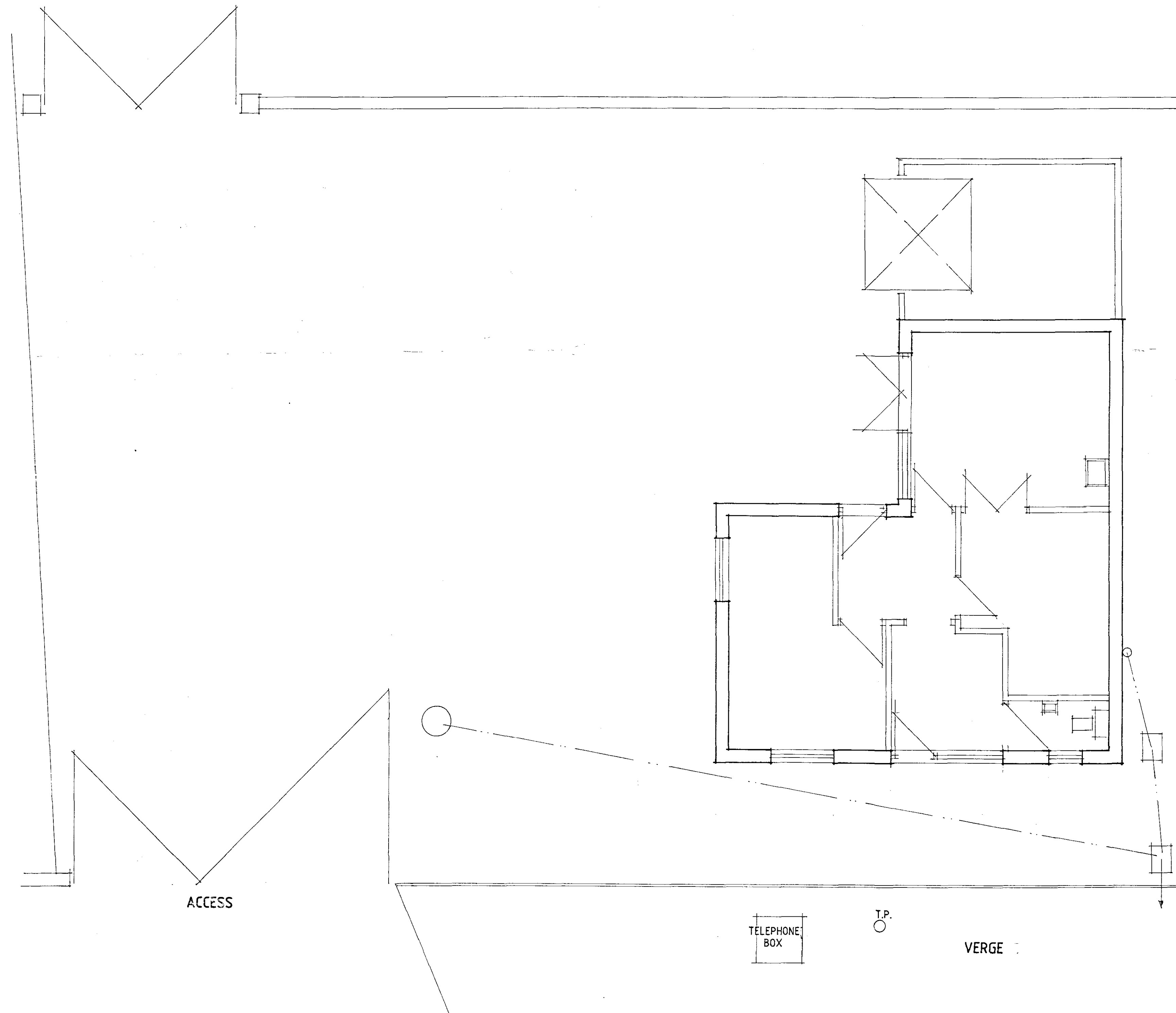
FLOOR PLAN
