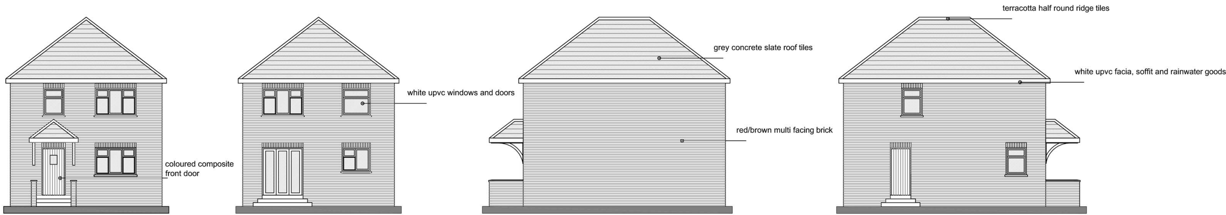
PROPOSED ELEVATIONS
