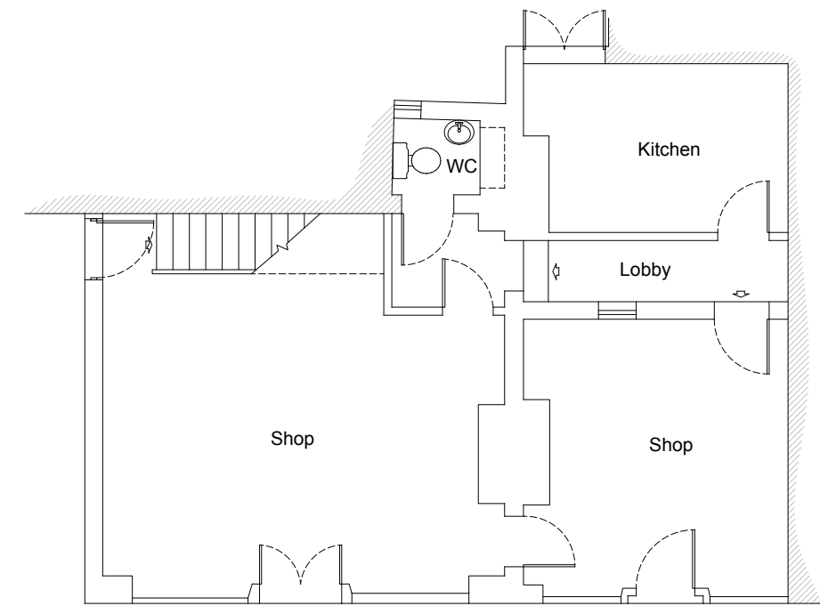
Ground Floor Plan 1:100 EXISTING
