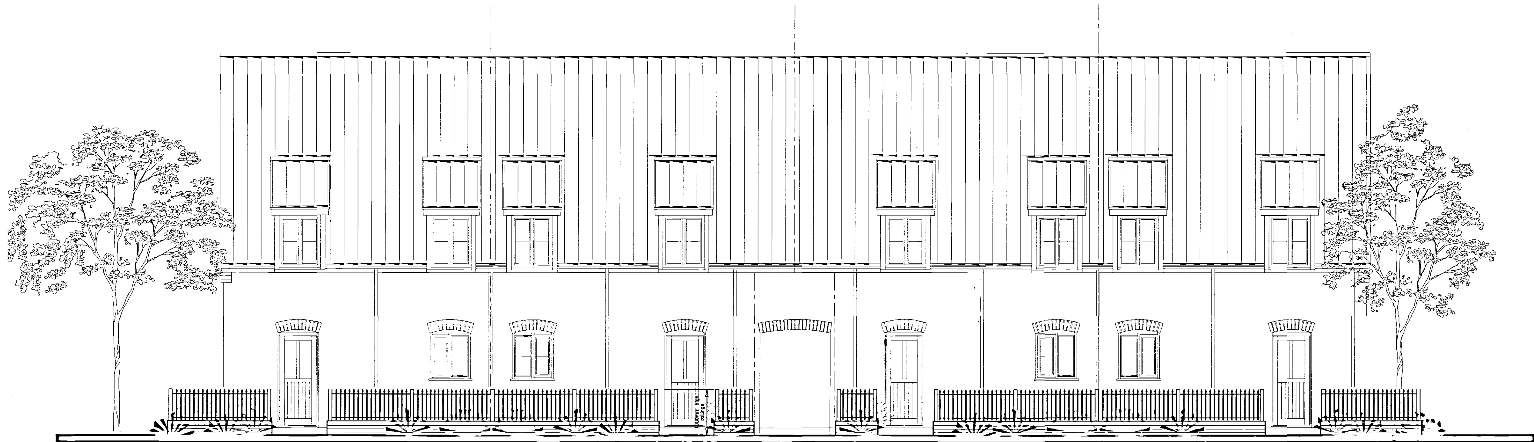
PROPOSED FRONT (EAST) ELEVATION DWELLINGS - 9 - 16 scale: 1:50
