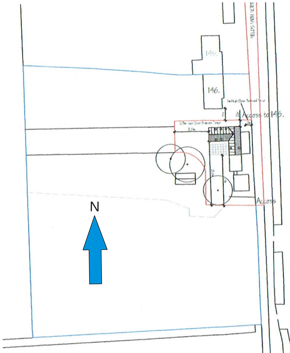
Figure 4: Block plan showing the proposed layout of the development site at an original scale of 1:500, (not to scale), (extract from Architects plan)
