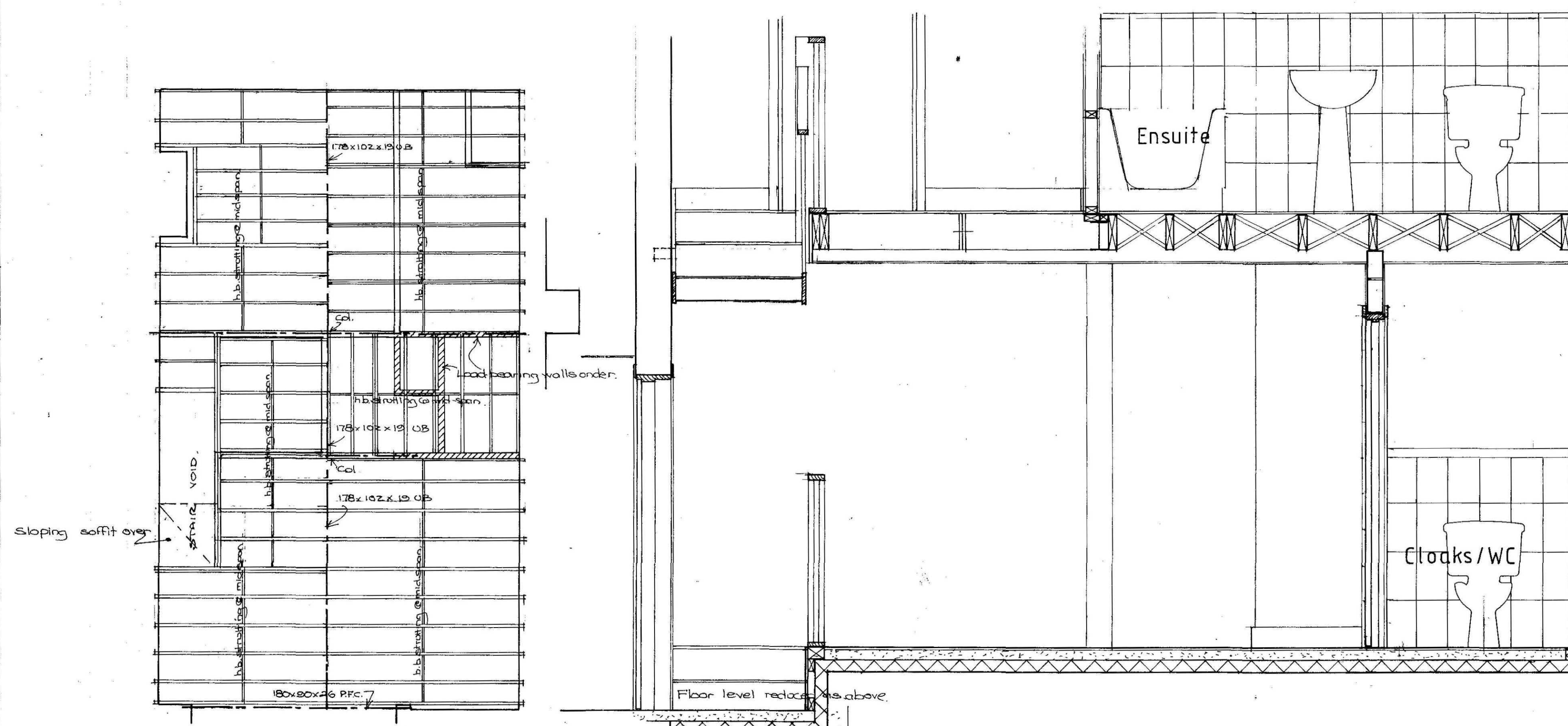
PLAN OF FIRST FLOOR STRUCTURE 1:50
