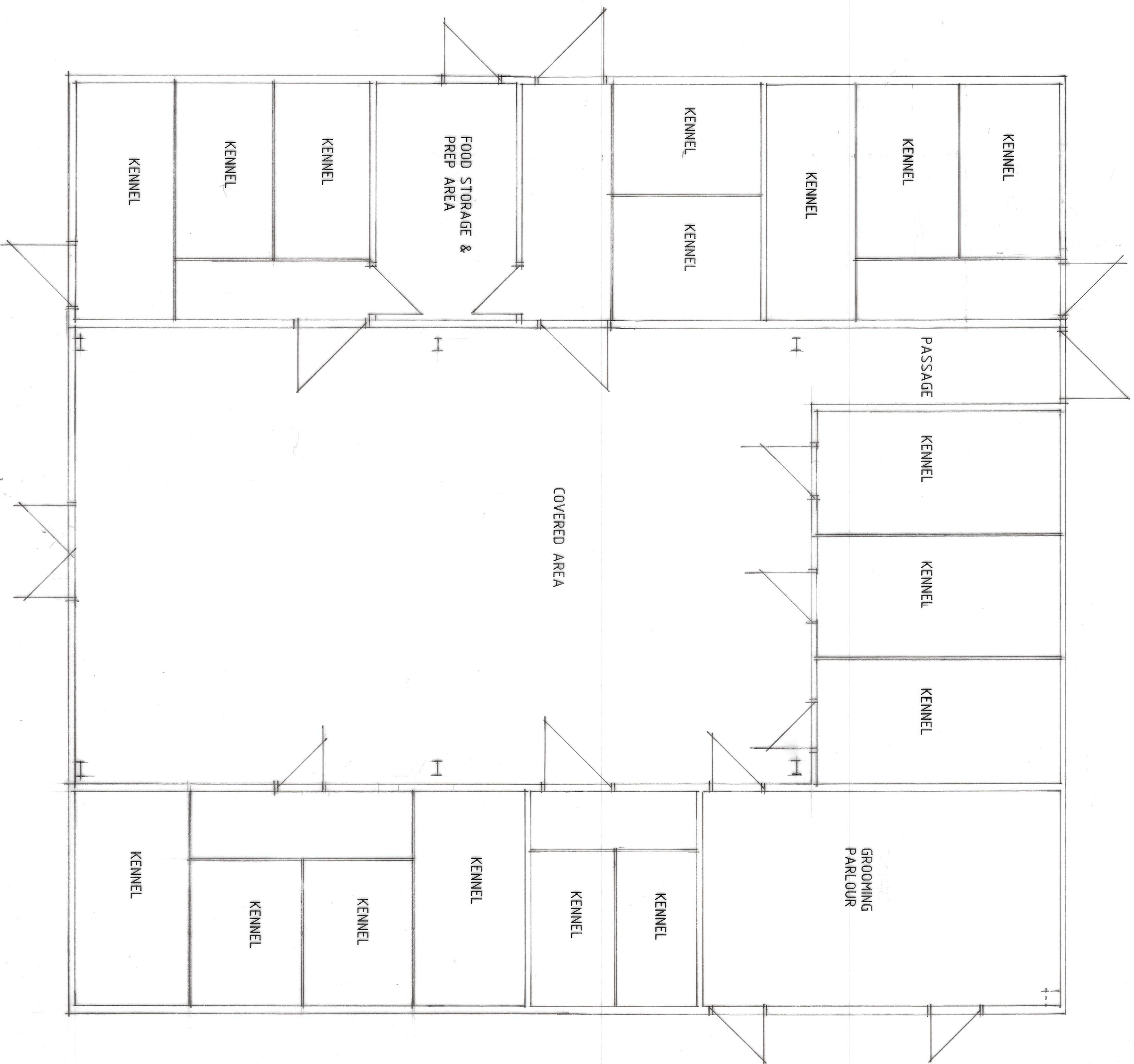
FLOOR PLAN
