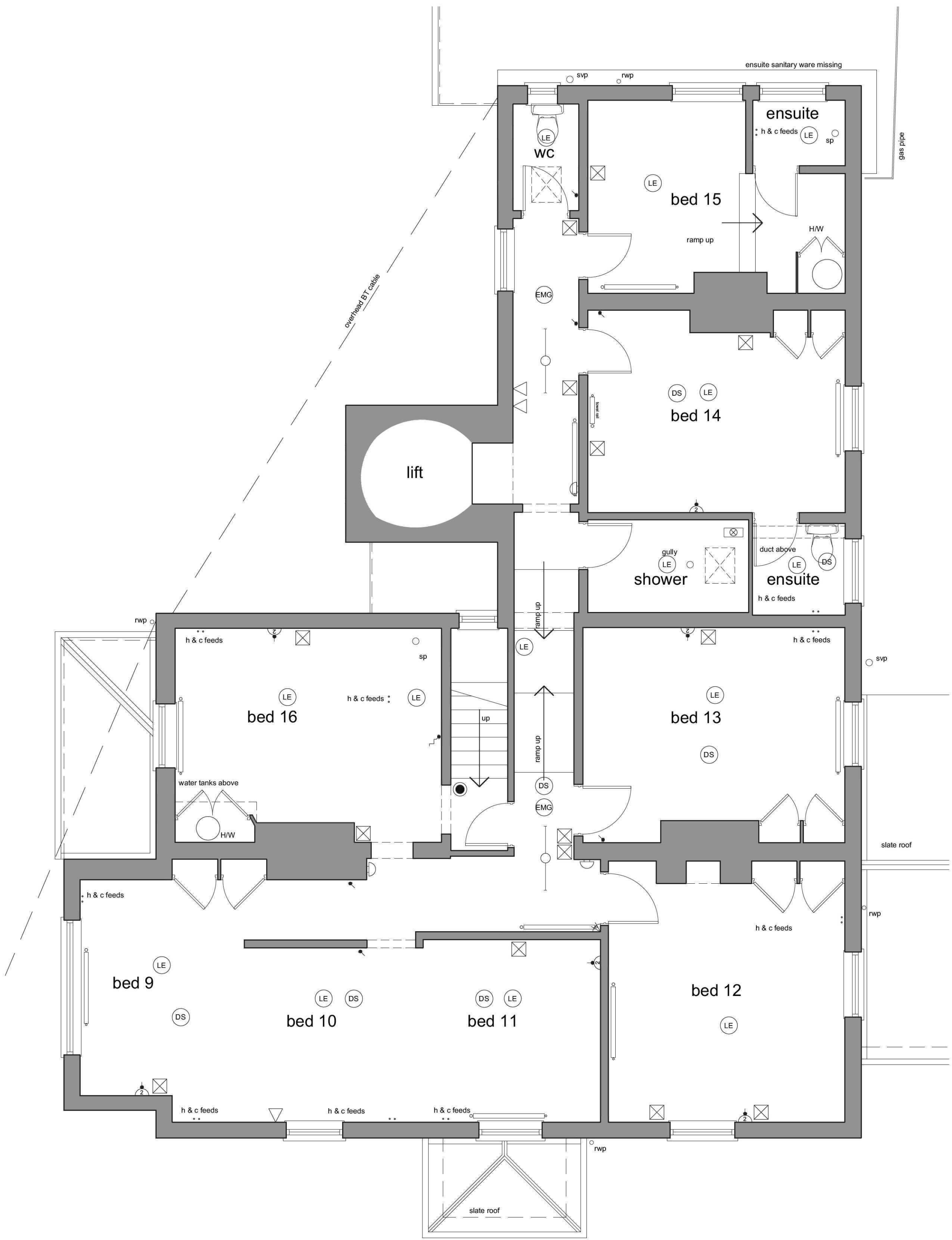
First Floor Services Layout Scale: 1:50
