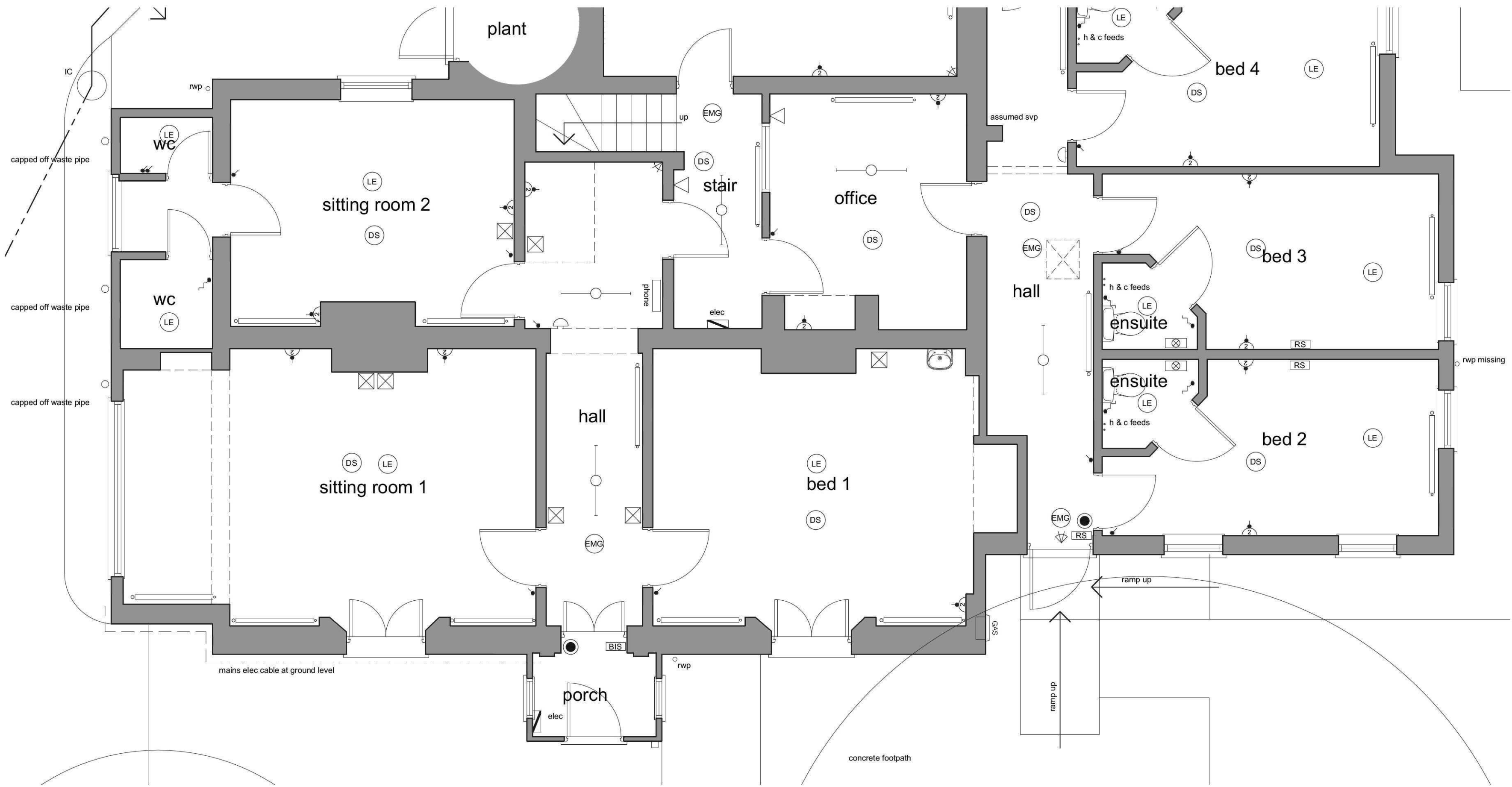
Ground Floor Services Layout (Part 2) Scale: 1:50
