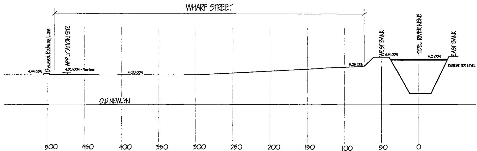
CROSS SECTION
