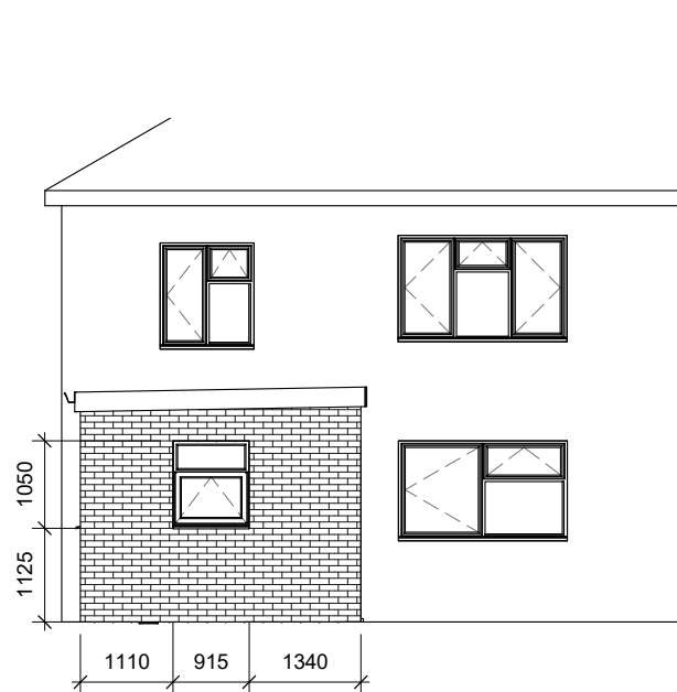
1 Proposed SW Elevation 1 : 100
