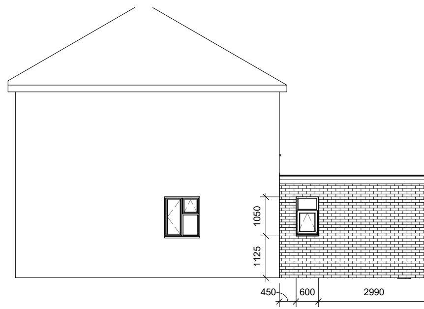
2 Proposed NW Elevation 1 : 100
