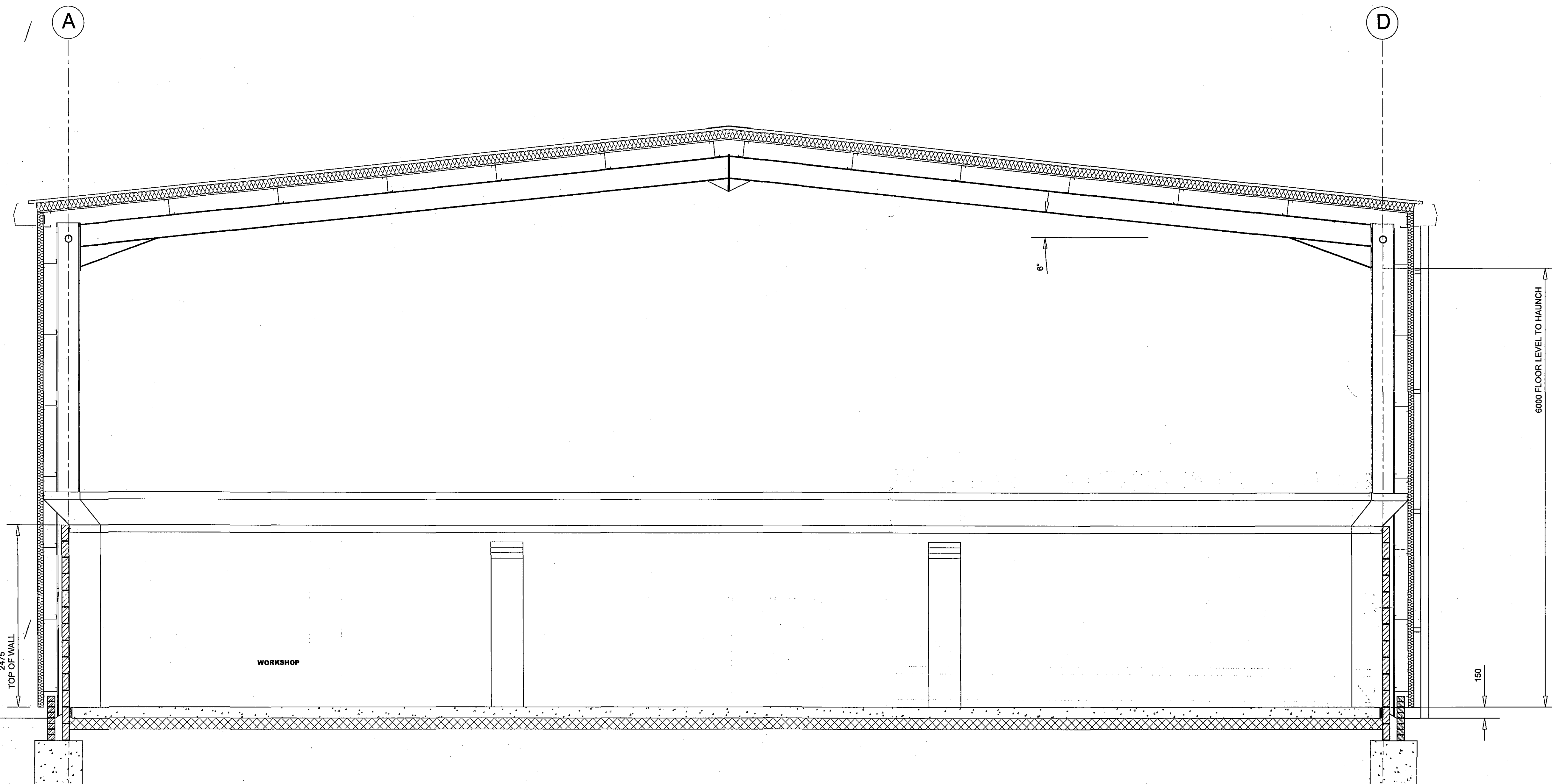
SECTION B ~ B scale 1:50
