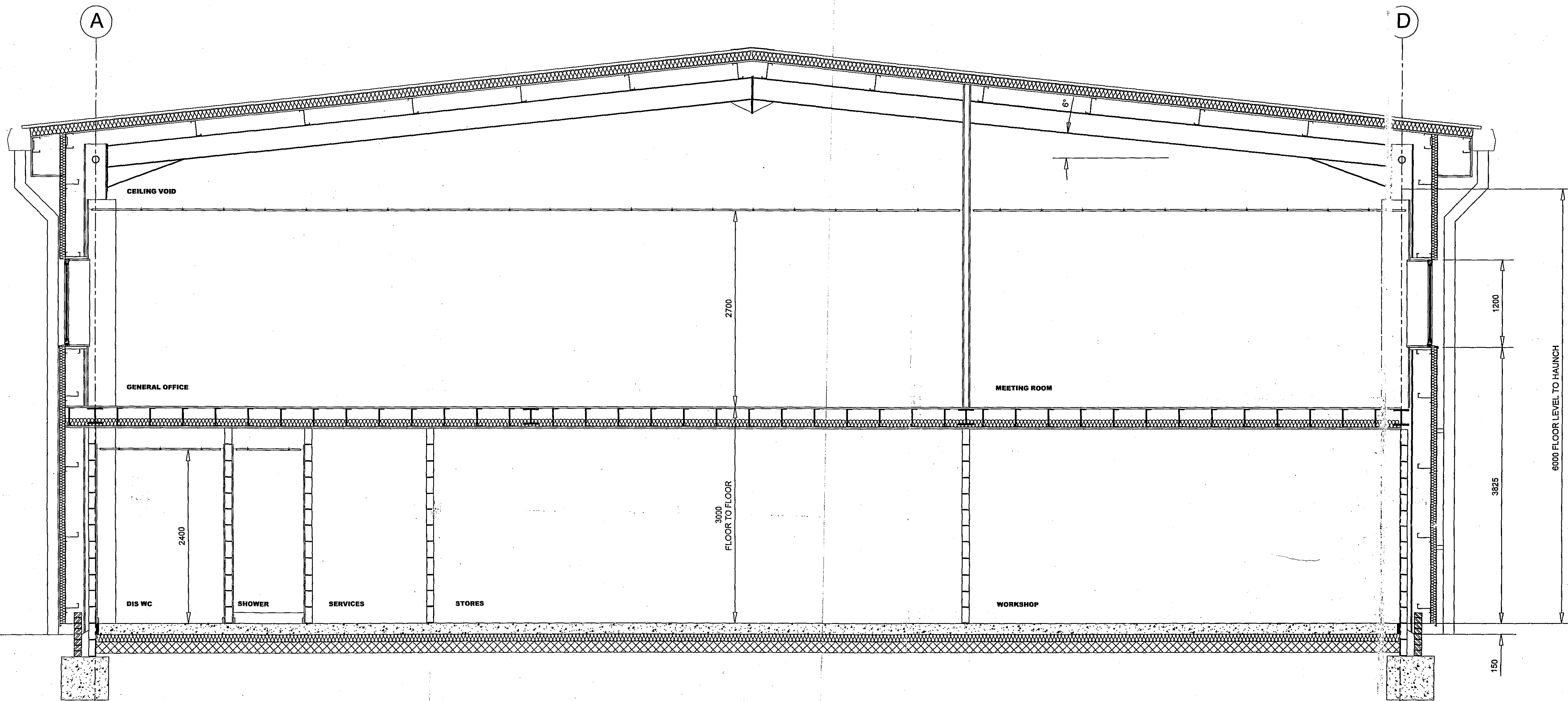
SECTION A ~ A scale 1:50
