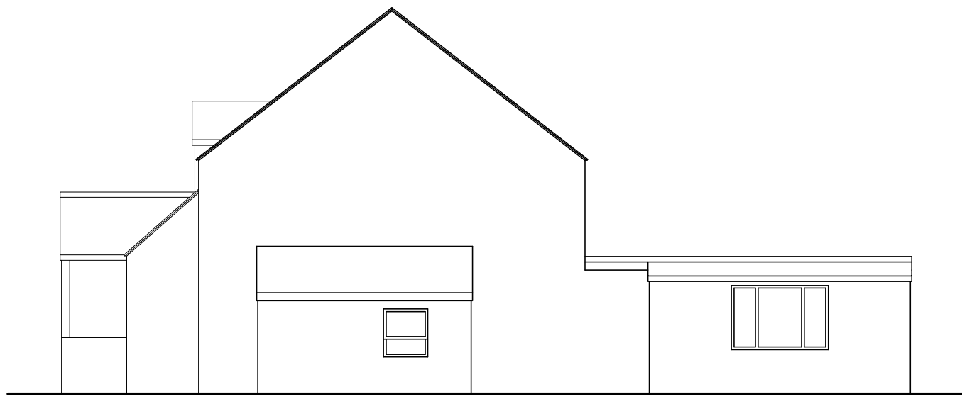
Existing Side elevation (North) 1:100
