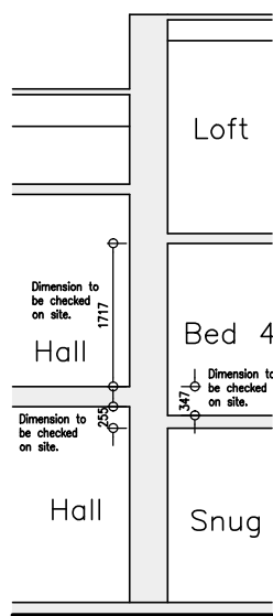
Existing Section C-C 1:100
