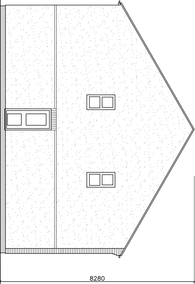
SIDE PROPOSED
