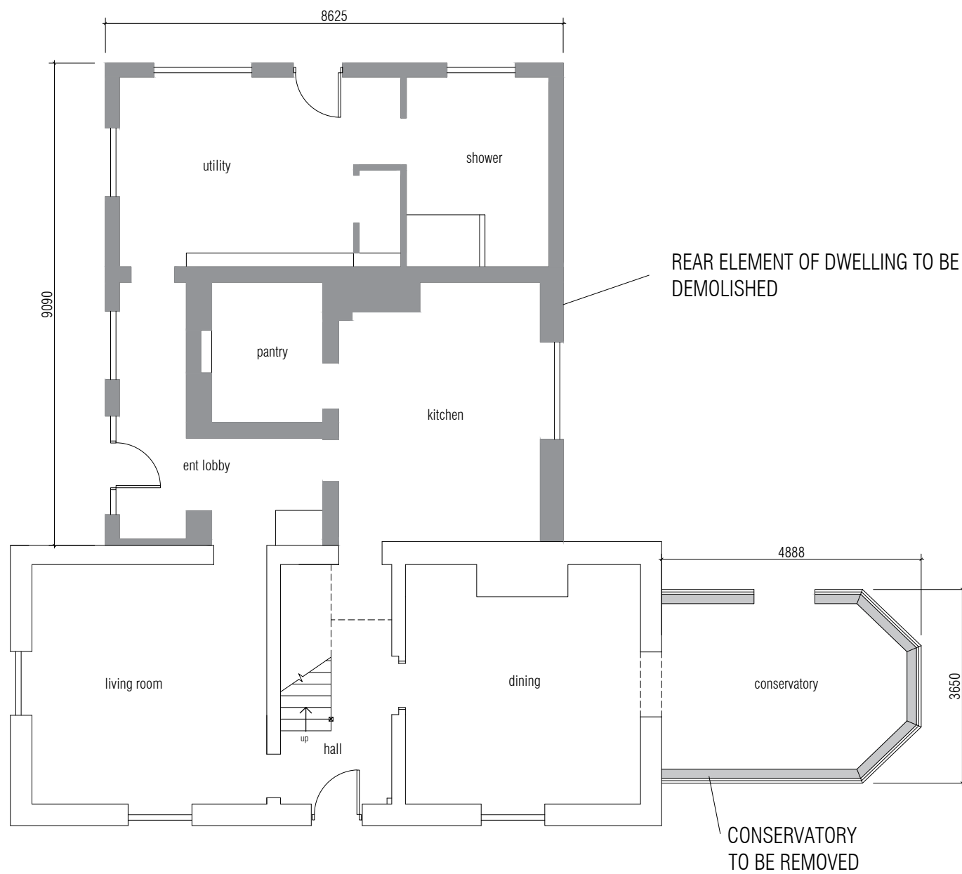
Ground Floor Layout as existing
