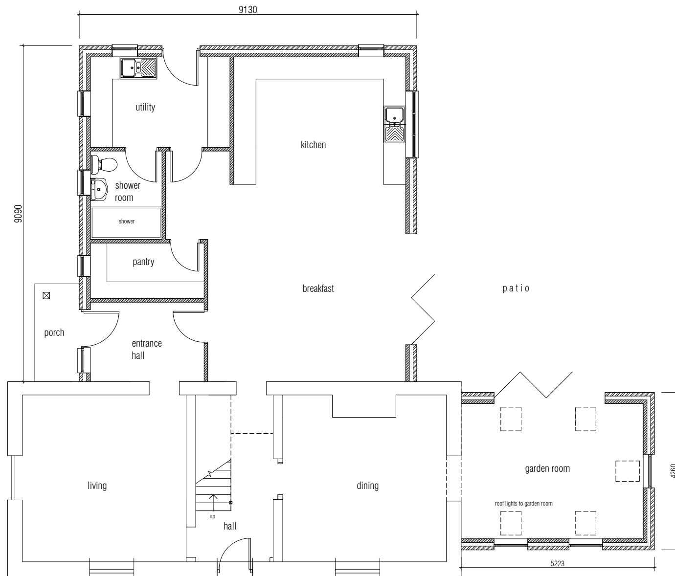
Ground Floor Layout - as proposed
