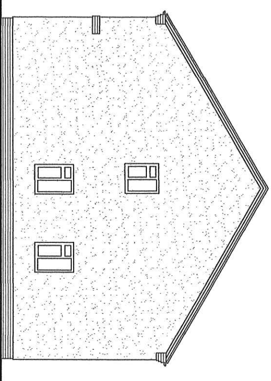
SIDE PROPOSED
