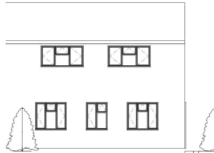
2 East Elevation - (Proposed) 1 : 100
