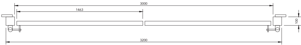
PLAN ELEVATION
