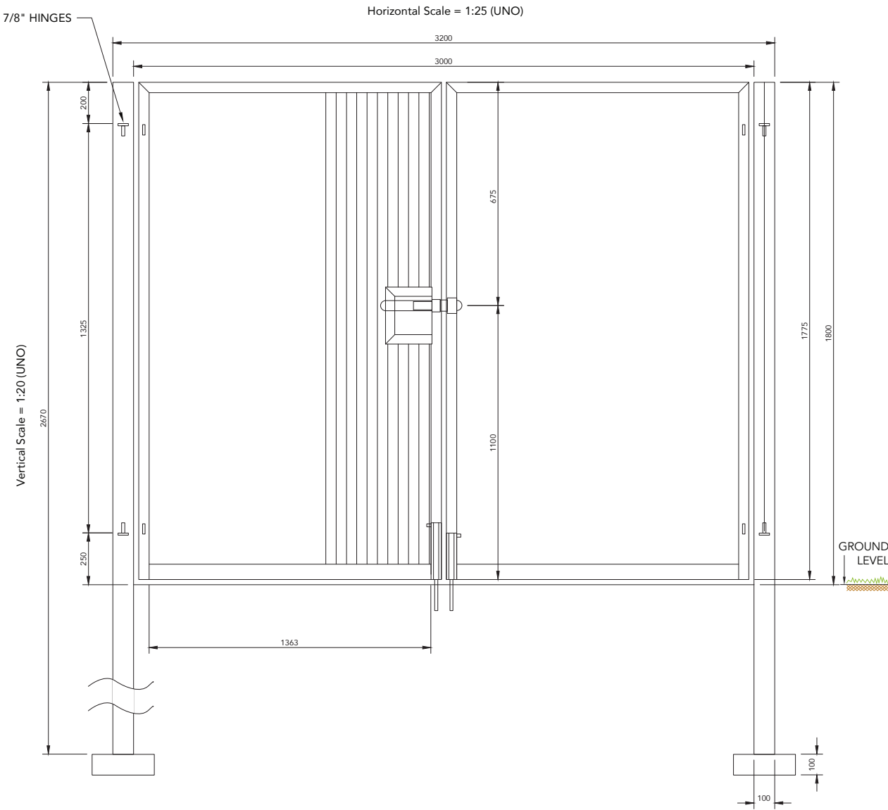
SIDE ELEVATION
