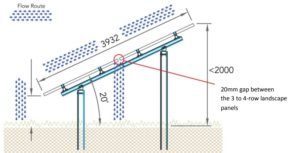
Example of Flow Route – (Property of BE Renewables Limited)
