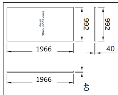
EXAMPLE OF TYPICAL 72 CELL SOLAR MODULE – IN LANDSCAPE ORIENTATION
