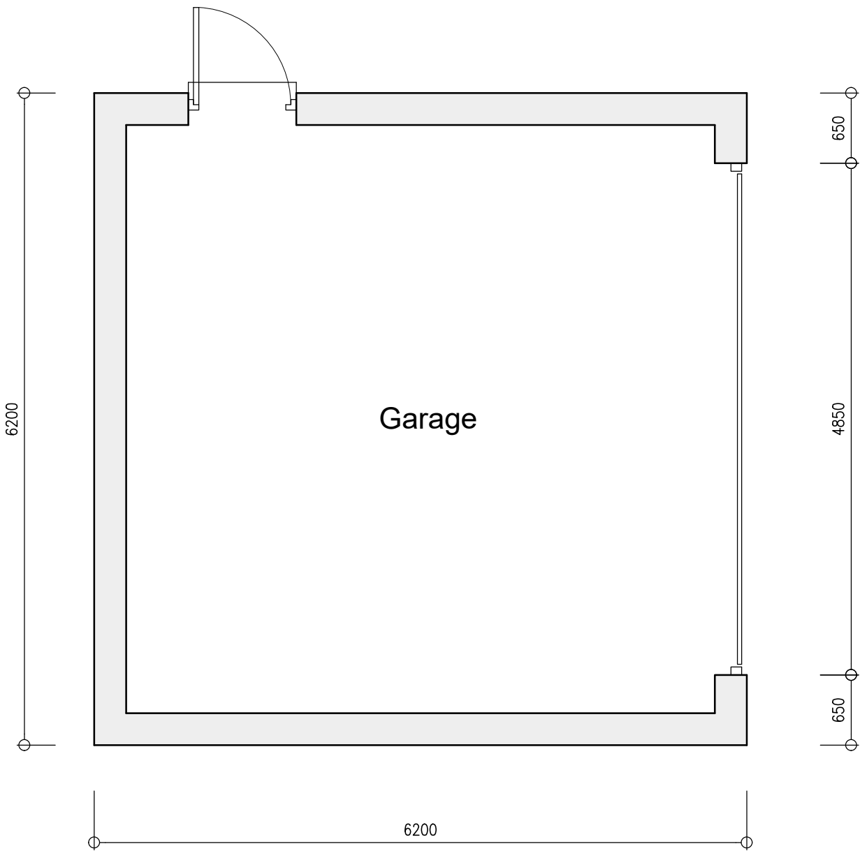
PROPOSED GROUND FLOOR SCALE 1:50
