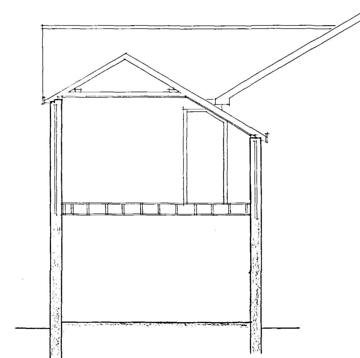
SECTION B-B
