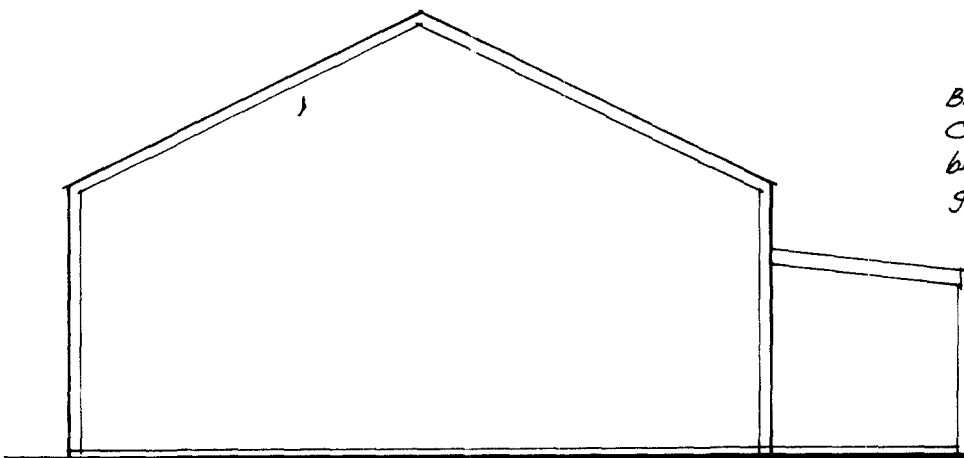
Rear. Elevations.
