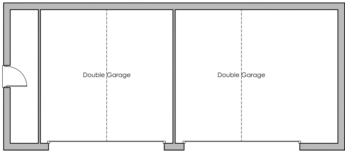
Floor Plan 1:100
