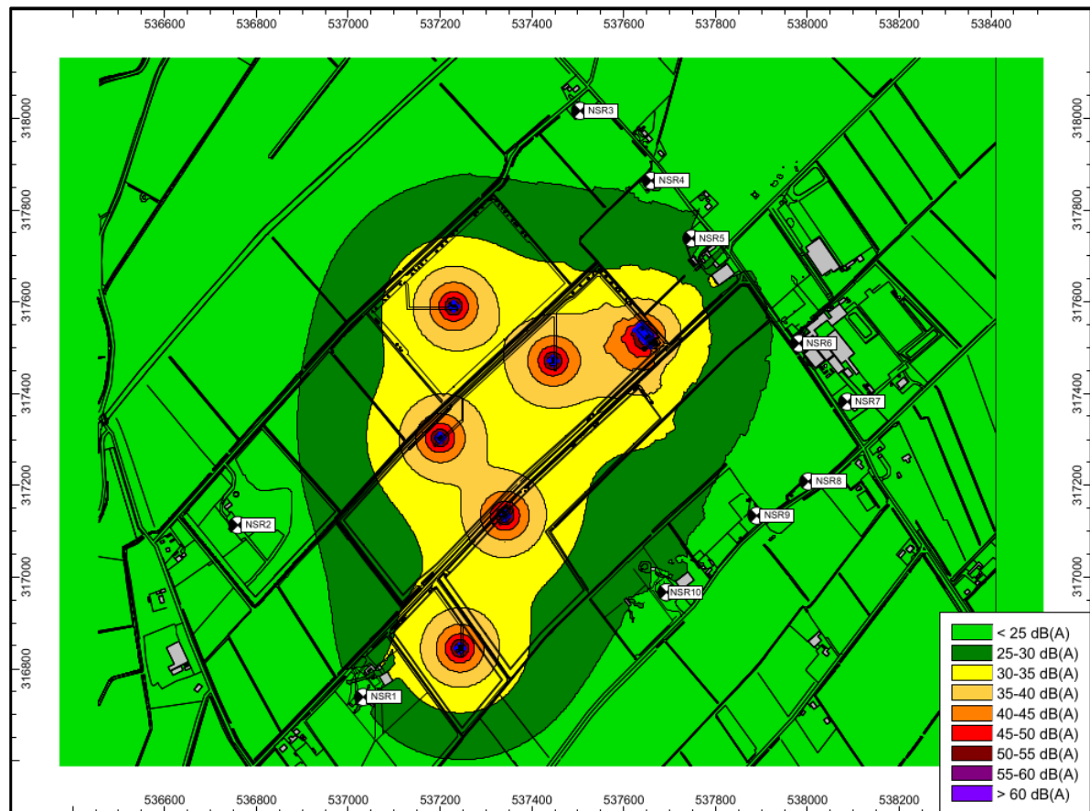
FIGURE 5: SPECIFIC SOUND LEVEL MAP - DAYTIME
