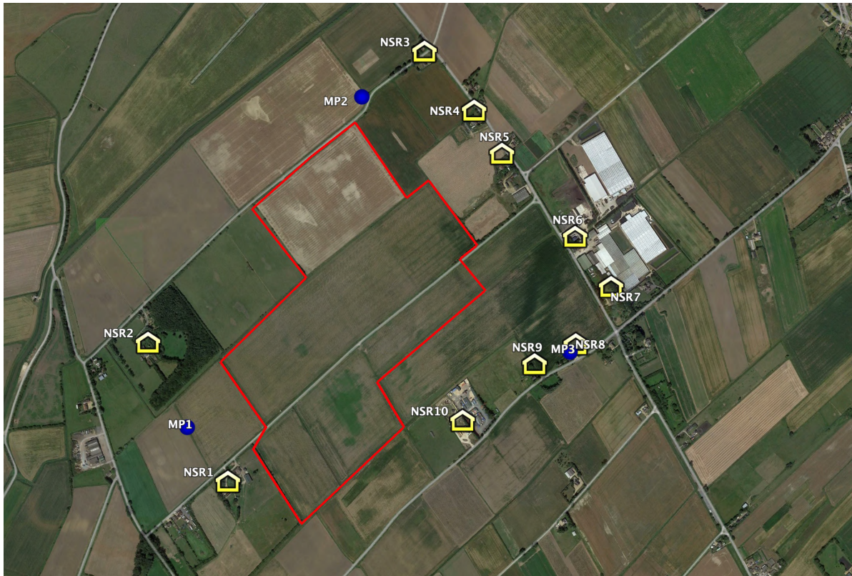
FIGURE 3: MEASUREMENT POSITIONS
