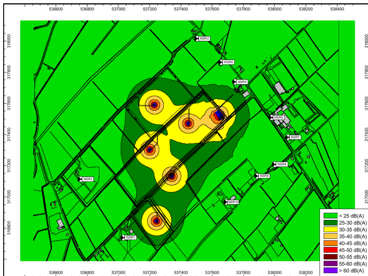
FIGURE 6: SPECIFIC SOUND LEVEL MAP – NIGHT-TIME
