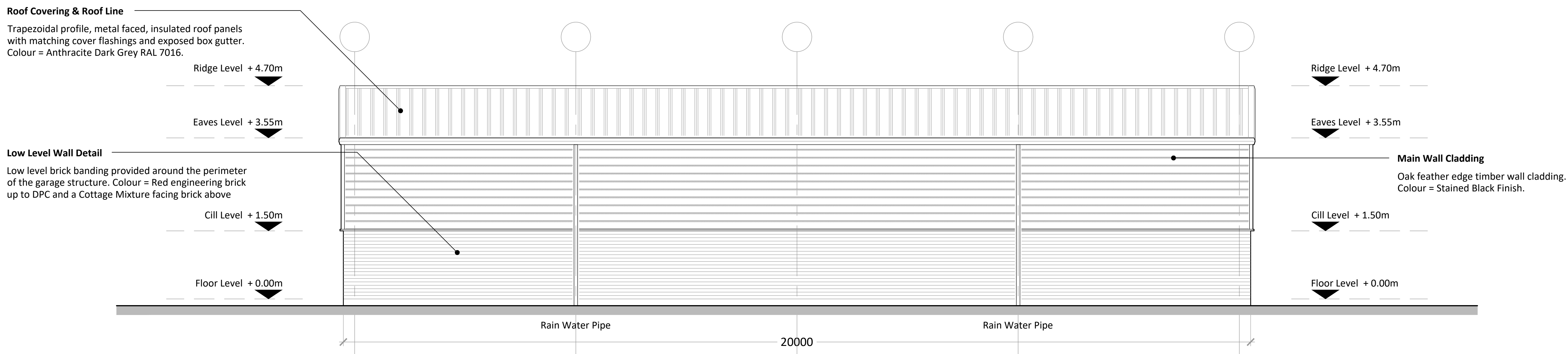
Proposed Rear Elevation (South facing)
