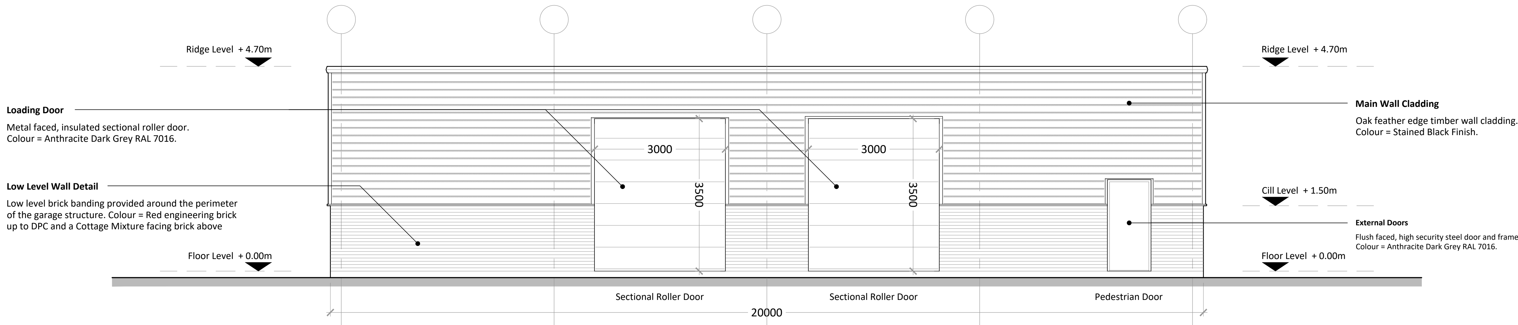
Proposed Front Elevation (North facing)
