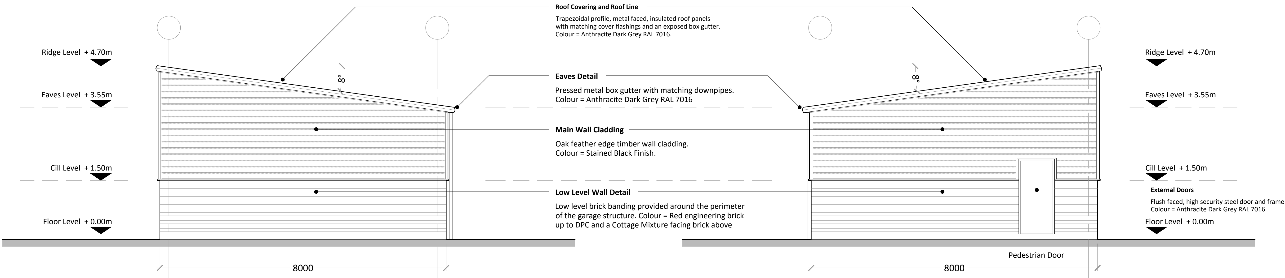
Proposed Side Elevation - A (West facing)
