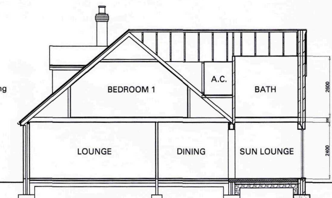
PROPOSED SECTION
