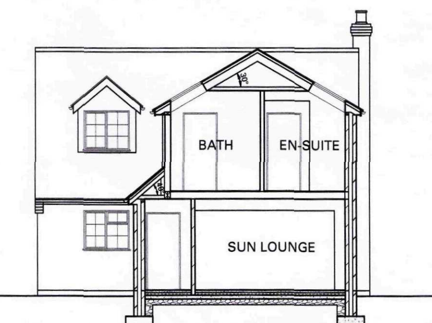
PROPOSED SECTION
