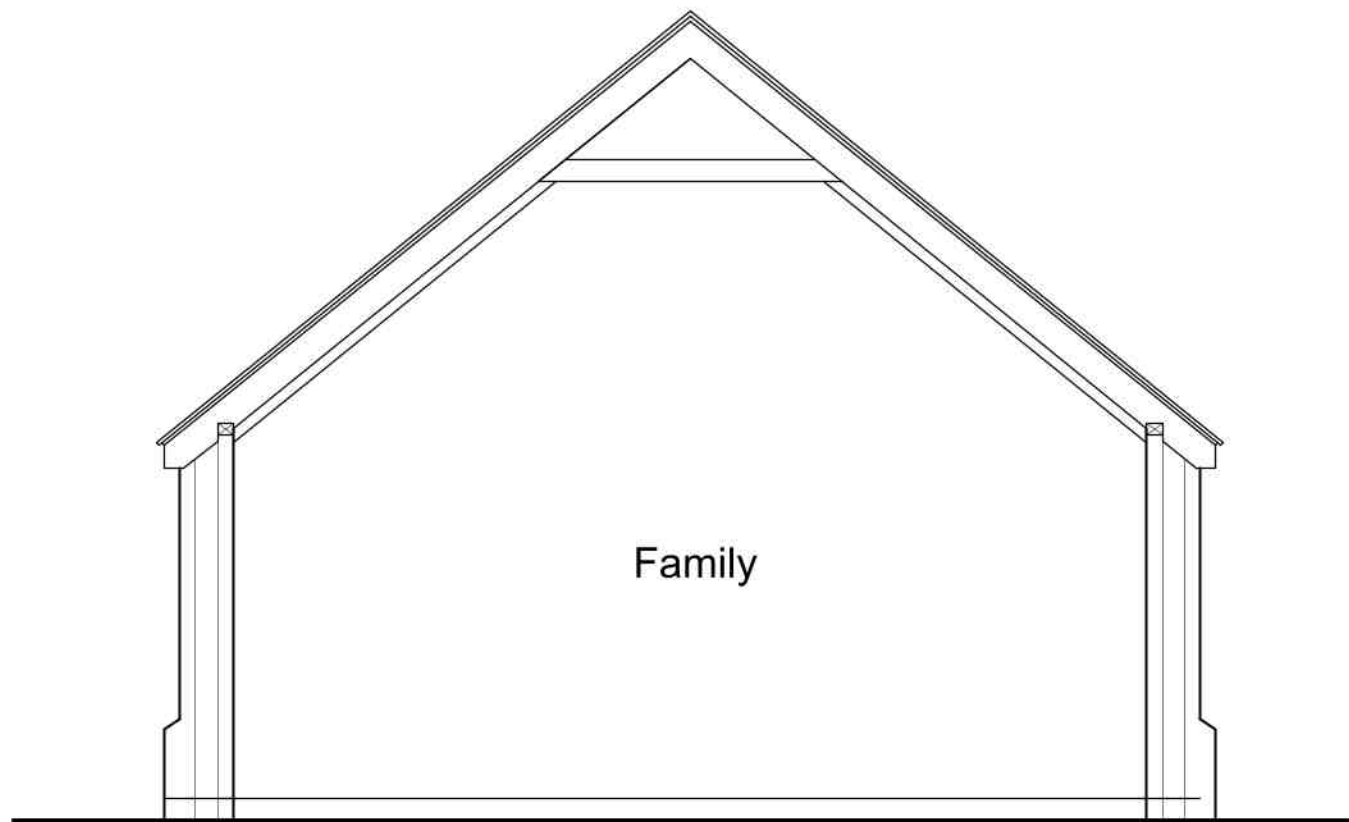
Section Thru' 1:50
