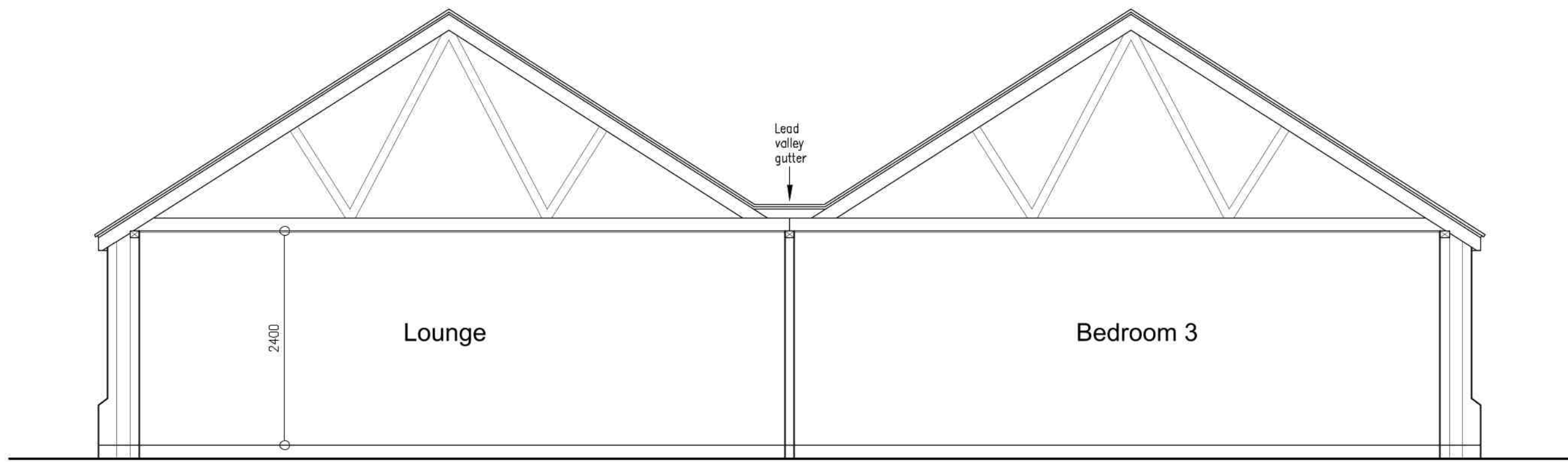
Section Thru' 1:50
