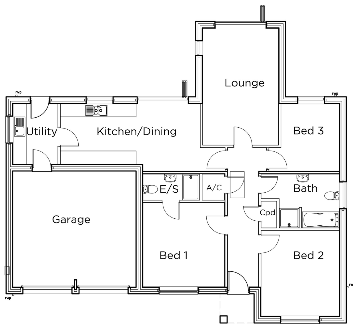
Ground Floor Plan Plot 4
