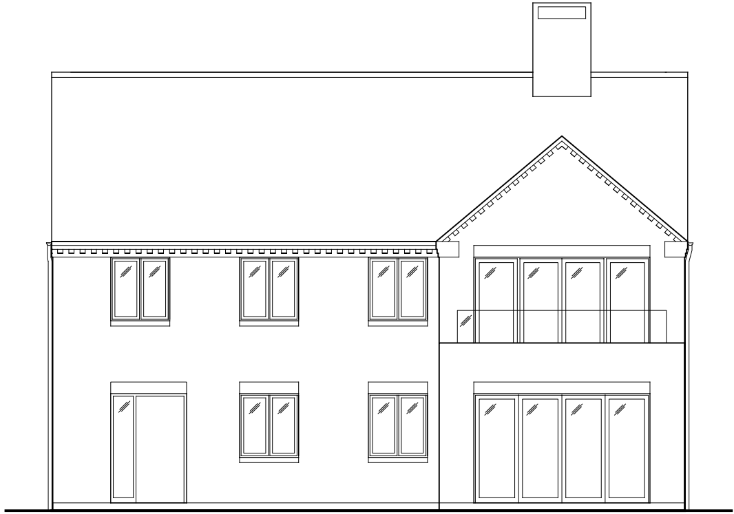
West Elevation
