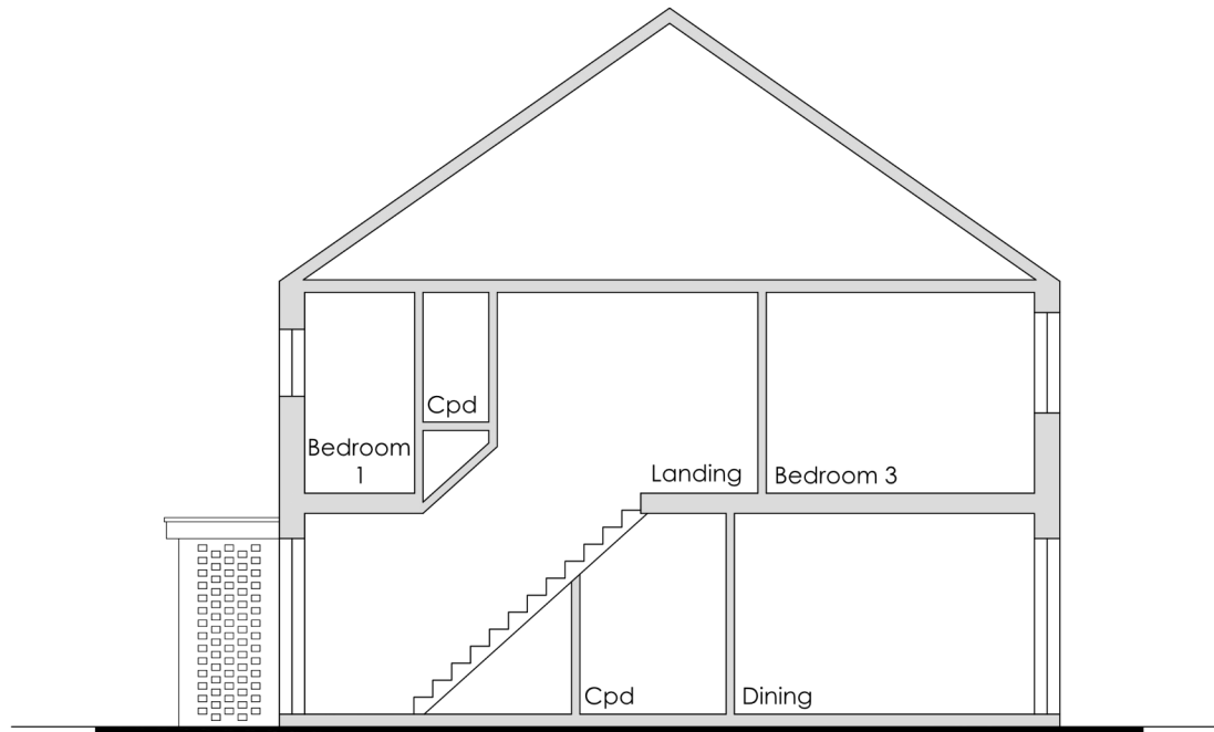
Typical Section
