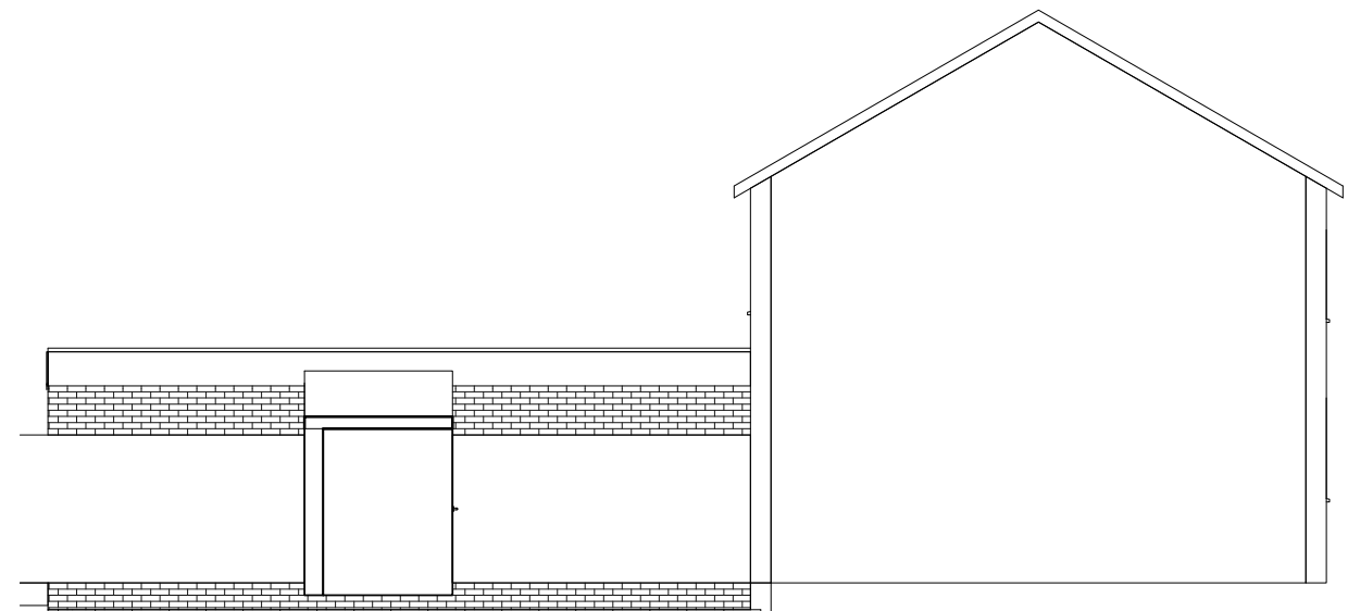
3 NE Elevation - (Proposed) 1 : 100
