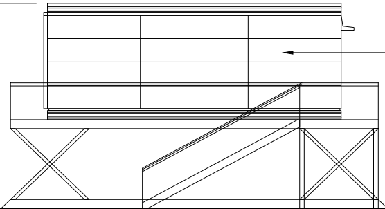
East Elevation
