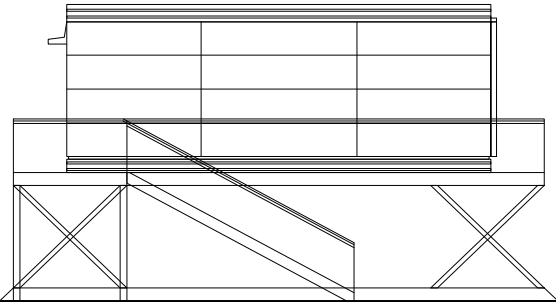
West Elevation
