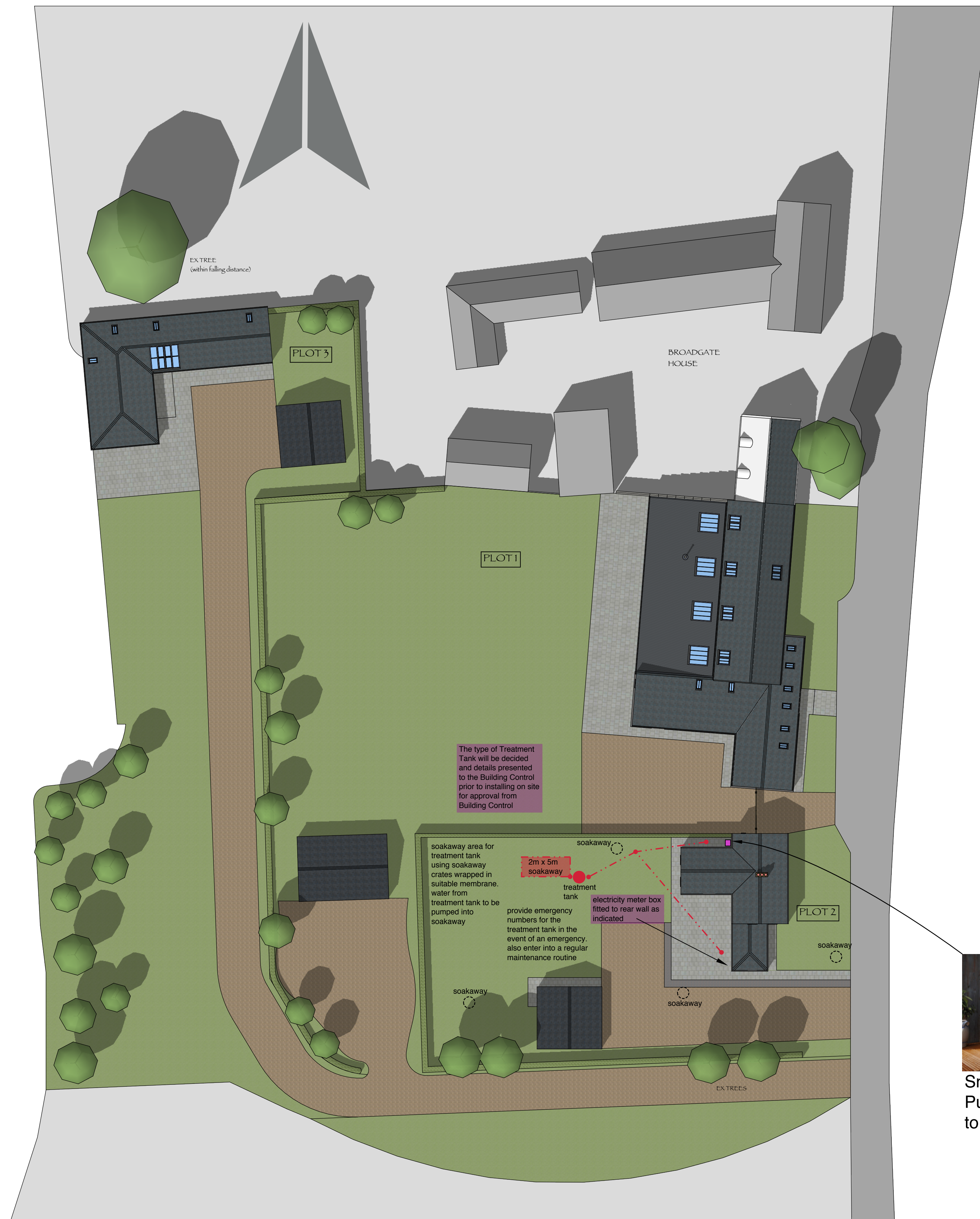
BLOCK PLAN
